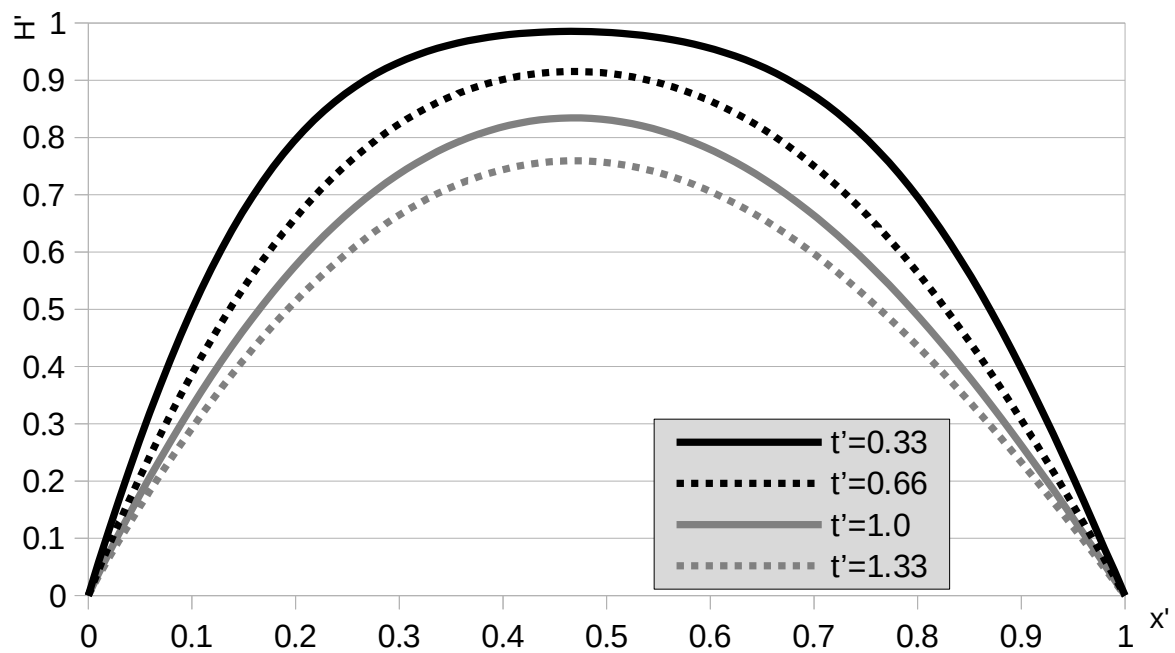
Figure 1. Dimensionless concentration C' = \frac{C}{C_0} (a) and water head H' = \frac{H}{H_0} , P = H * g where P is the pore pressure (b) depending on dimensionless space variable x' = \frac{x}{x_0} in the dimensionless moments of time t' = \frac{t}{t_0} for \alpha = 0.9 , \beta = 0.8 , C_0 = 200 g/L, H_0 = 10 m, x_0 = 25 m, t_0 = 60 days.
