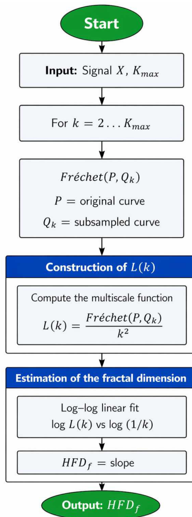
Figure 2. HFDf estimate flowchart. Starting from the original sEEG signal, sub-sampled traces are generated at increasing values of the down-sampling factor k (with 2 \leq k \leq K_{max} ). For each k , the Fréchet distance is computed between the sub-sampled trace and the full original trace used as reference. HFDf is then estimated as the slope of \log(L(k)) versus \log(1/k) , replacing the Euclidean curve length with the Fréchet-based distance. Code and pseudocode can be found at https://github.com/ceconifederico/HDFf_tool (accessed on 10 June 2026).
