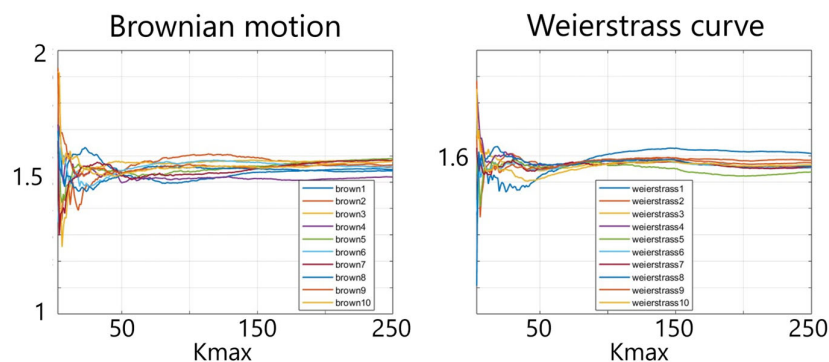
Figure 3. HFDf(Kmax) for 10 synthetically generated Brownian motion and Weierstrass curve sequences.
