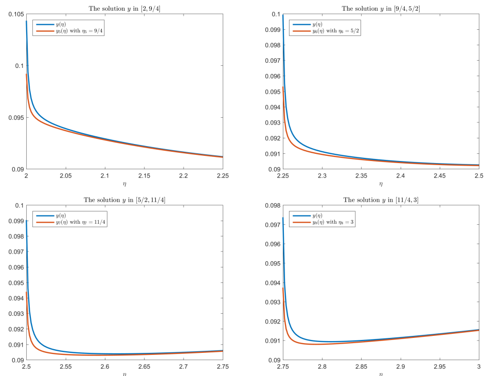
Figure 2. Comparison between the variable-order numerical solution y(\eta) and the piecewise-constant order solutions y_i(\eta) .
