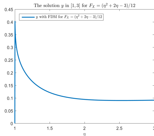
Figure 1. Numerical solution y(\eta) corresponding to F_X(\eta) = \frac{1}{12}(\eta^2 + 2\eta - 3) .
