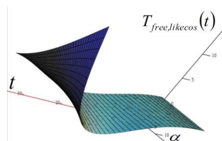
Figure 4. Surface of the self-eigen-time mode “like cos”, longitudinal flow of the rheological viscoelastic Maxwell model of a fractional-type material in a pipe, presented in the coordinate system of the amplitude of the self-eigen mode T_{free,likecos}(t) , time t , and exponent \alpha of the fractional-order derivative, on the interval 0 < \alpha \leq 1 , drawings from another direction of visibility.
