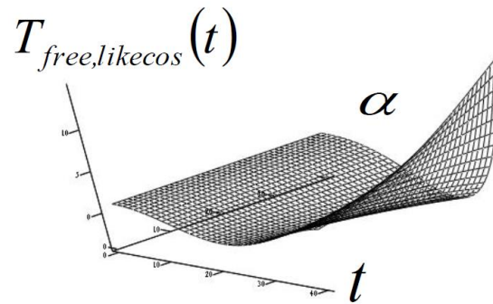
Figure 5. Surface of the self-eigen-time mode “like cos”, longitudinal flow of the rheological viscoelastic Maxwell model of a fractional-type material in a pipe, presented in the coordinate system of the amplitude of the self-eigen mode T_{free,likecos}(t) , time t , and exponent \alpha of the fractional-order derivative, on the interval 0 < \alpha \leq 1 , drawings from another direction of visibility and in black and white.
