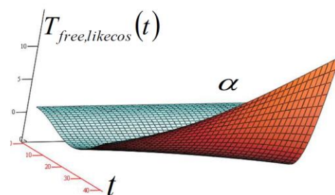
Figure 3. Surface of the self-eigen-time mode “like cos”, longitudinal flow of the rheological viscoelastic Maxwell model of a fractional-type material in a pipe, presented in the coordinate system of the amplitude of the self-eigen mode T_{free,likecos}(t) , time t , and exponent \alpha of the fractional-order derivative, on the interval 0 < \alpha \leq 1 .
