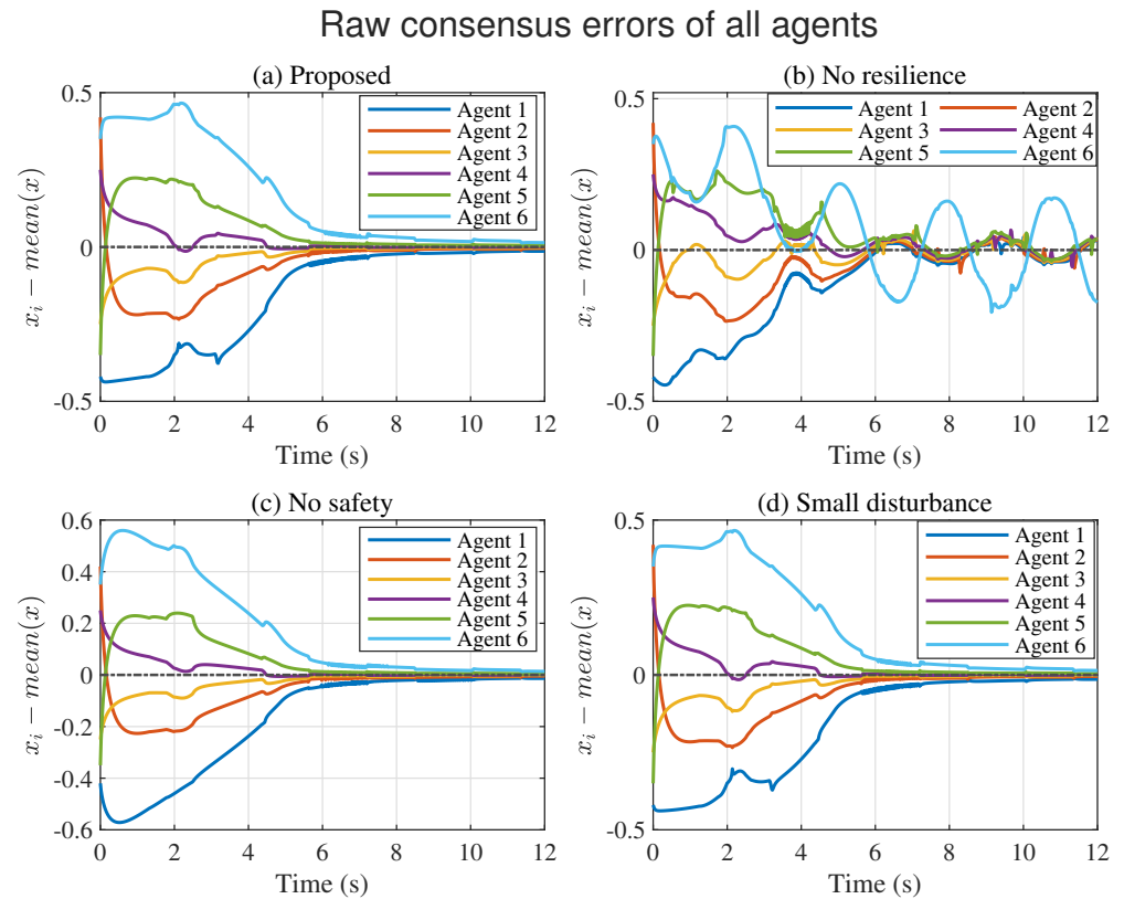
Figure 6. Raw consensus errors under different cases.
