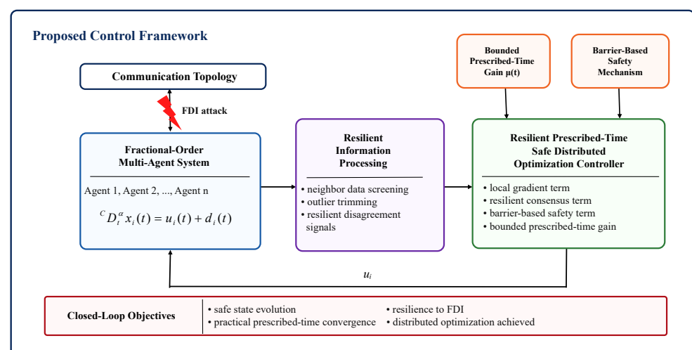
Figure 1. Overall control framework of the resilient safe distributed optimization method.
