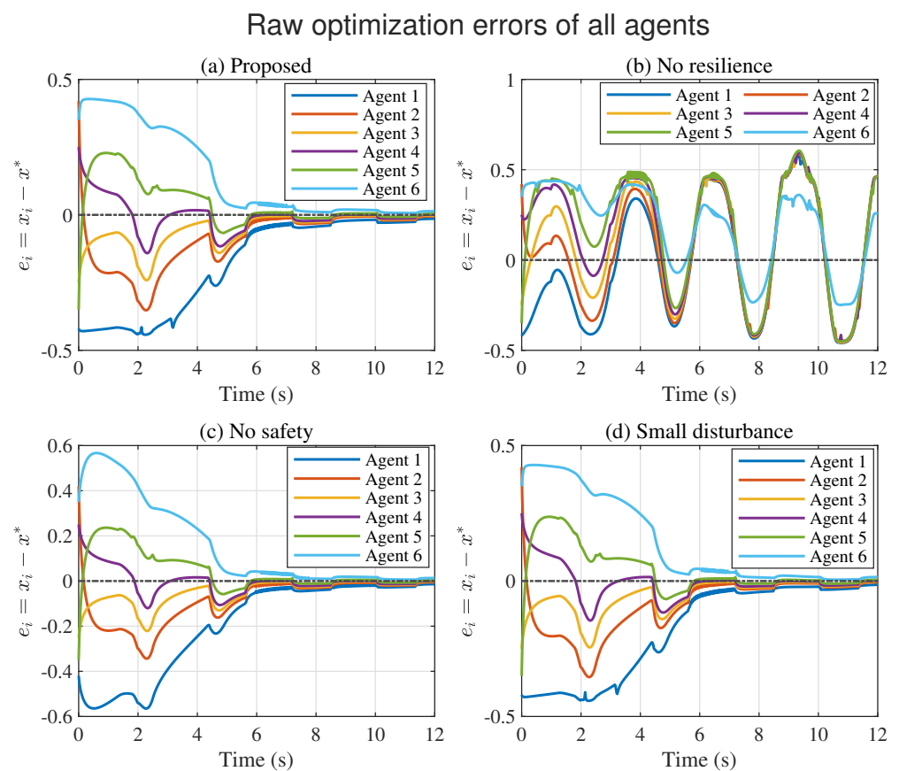
Figure 5. Raw optimization errors under different cases.
