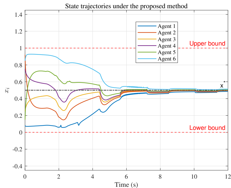
Figure 4. State trajectories under the proposed method.
