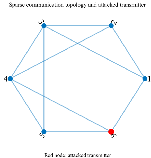
Figure 2. Communication topology under FDI attacks.
