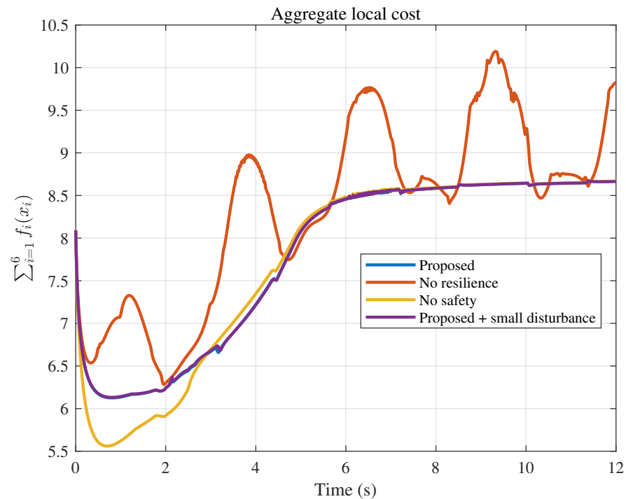
Figure 10. Aggregate local cost under different cases.
