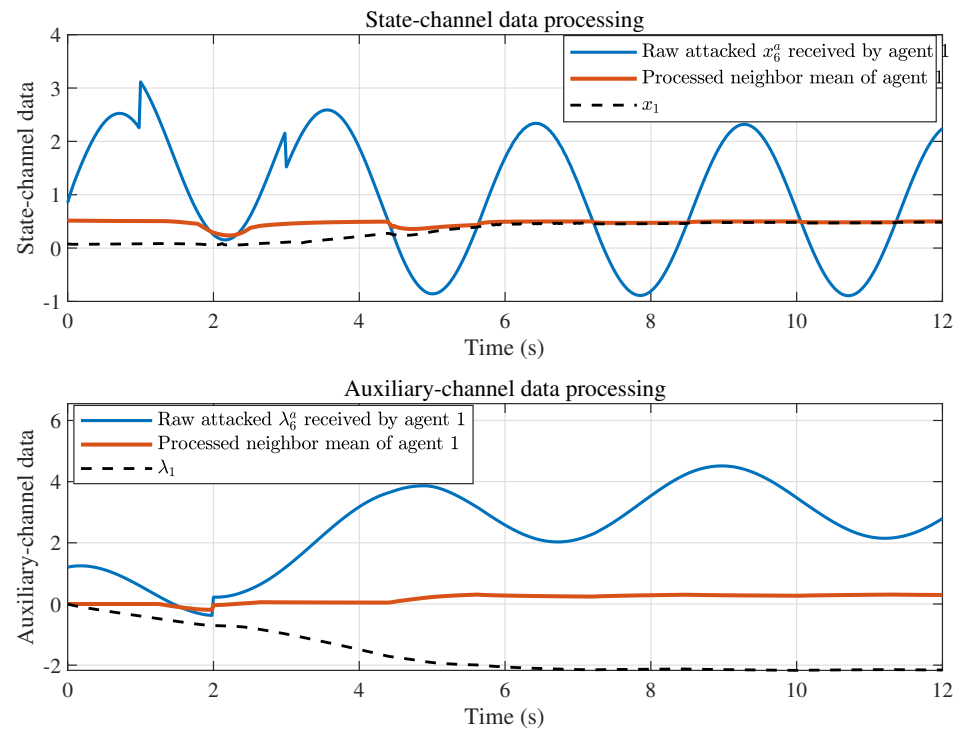
Figure 8. Effect of resilient information processing on corrupted neighboring data.
