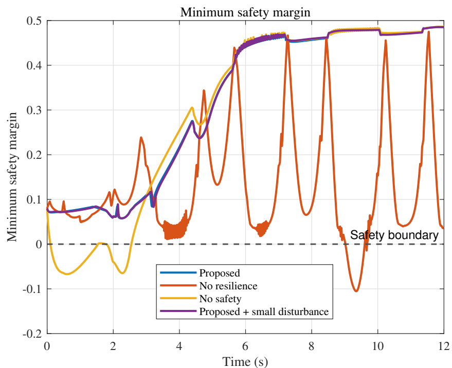
Figure 7. Minimum safety margin under different cases.
