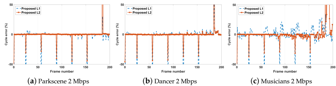
Figure 3. An illustration of the frame-wise percentage error between the target decoding-complexity and the achieved decoding-complexity for the proposed algorithm at two complexity levels for a given bit rate (2 Mbps) for (a) Parkscene, (b) Dancer and (c) Musicians test sequences.
