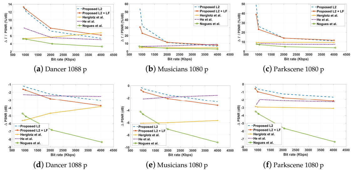
Figure 4. An illustration of the variation of the \Delta\Gamma , \Delta PSNR ratio (top row), i.e., \widetilde{\Delta\Gamma} (%/dB), and \Delta PSNR (bottom row), with respect to the bit rate.
