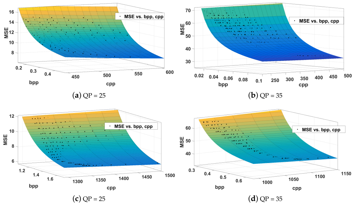
Figure 1. The decoding-complexity (cpp), rate (bpp) and distortion (MSE) behavior of inter-predicted (top row) and intra-predicted (bottom row) frames.
