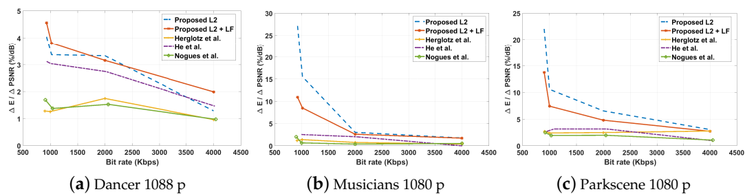
Figure 6. An illustration of the variation of the \Delta E , \Delta PSNR ratio, i.e., \widehat{\Delta E}(\%/dB) , with respect to the bit rate for (a) Dancer, (b) Musicians and (c) Parkscene HD test sequences.
