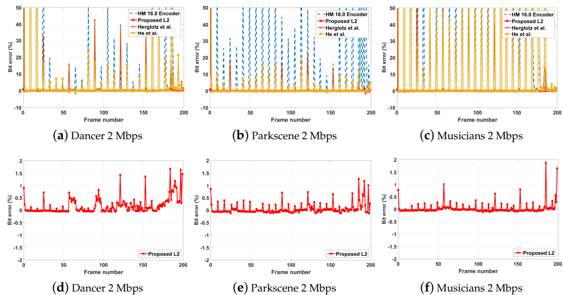
Figure 2. (Top row): An illustration of the frame-wise percentage error between the allocated bits and actual bits for the HM 16.0, proposed, and other state-of-the-art algorithms for three HD test sequences. (Bottom row): A further illustration of the percentage frame-wise rate control performance of the proposed algorithm.
