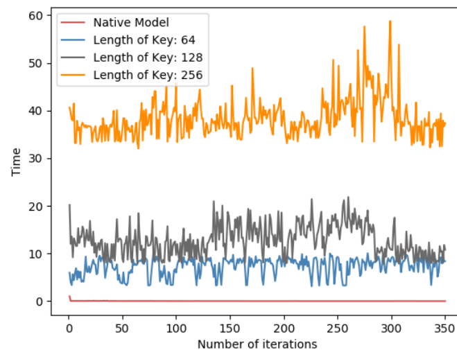
Figure 9. Per-iterations time spent for different key lengths on the fatigued dataset.
