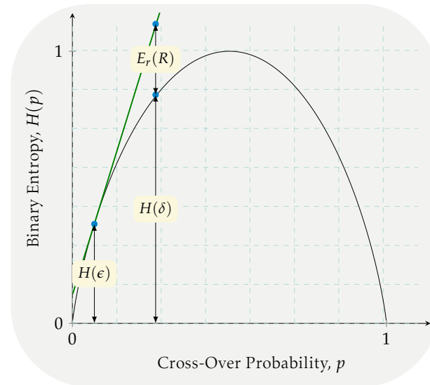
Figure 7. Depiction of the error exponent for a BSC. The tangent line of the binary entropy function H(p) in the cross-over probability point 0 < p = \epsilon < 1/2 , calculated for \epsilon < p = \delta < (1 - \beta)\epsilon + \beta/2 , marked in green, is denoted by T_\epsilon(\delta) . For a given cross-over probability \epsilon , the difference between T_\epsilon(\delta) and H(\delta) is referred to as the error exponent. For example, the upper bounds on the goal identification rate \kappa calculated in (A58) and (A59) are two different error exponents that are derived in the sort II error analysis. The minimum of these error exponents is the bottleneck for the rate \kappa , i.e., an eligible upper bound.
