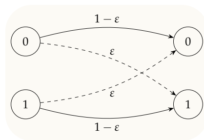
Figure 1. Bit transition graph over a BSC. Each bit is flipped independently of other bits, with a cross-over probability of \varepsilon \in (0, 1/2) .
