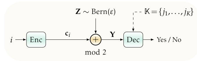
Figure 2. System model for DKI communication setting over a BSC. Employing a deterministic encoder at the transmitter, the message i is mapped to the codeword \mathbf{c}_i = (c_{i,t})_{t=1}^n using a deterministic function. The decoder at the receiver is provided with an arbitrary goal message set \mathbb{K} , and given the channel output \mathbf{Y} = (Y_t)_{t=1}^n , it asks whether or not i belongs to \mathbb{K} .
