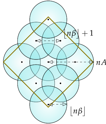
Figure 6. Illustration of an exhausted greedy-wise ball covering of an n -dimensional Hamming hyper ball \mathcal{B}_0(n, nA) , where the union of the small balls of radius r_0 = \lfloor n\beta \rfloor cover a larger Hamming hyper ball. As the codewords are assigned to the center of each ball lying inside the an n -dimensional Hamming hyper ball \mathcal{B}_0(n, nA) according to the greedy construction, the Hamming weight of a codeword is bounded by nA , as required.
