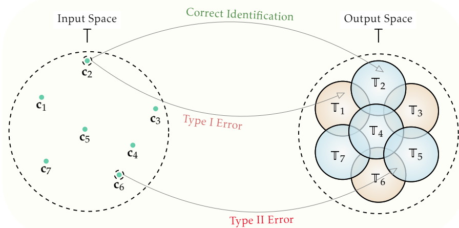
Figure 3. A DKI configuration with K = 4 and a goal message set \mathbb{K} = \{2, 4, 5, 7\} is displayed. The channel's output is located in the union of each individual decoder \mathbb{T}_j (marked in blue) in the correct identification event, where j is a member of the goal message set. If the channel output is seen in the complement of the union of distinct decoders that the codeword's index belongs to, a sort I error event takes place. When the transmitted codeword's index does not belong to \mathbb{K} , and the channel output is recognized in the union of the individual decoders \mathbb{T}_j , with j \in \mathbb{K} , an error event of sort II occurs.
