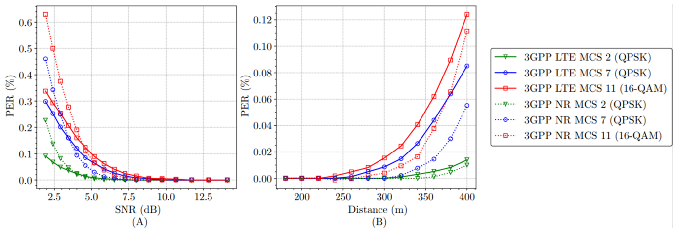
Figure 5. Comparison of (A) PER vs. SNR and (B) PER vs. distance for LTE-V2X and NR-V2X with payload of 375 bytes.
