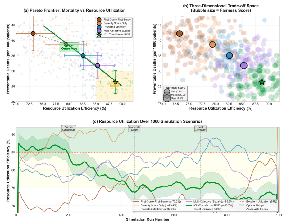
Figure 7. Resource allocation comparison strategies between prevention mortality reduction and resource utilization efficiency. Panel (a) illustrates the Pareto frontier between mortality and resource utilization efficiency, highlighting the trade-offs made by various models. Panel (b) shows the three-dimensional trade-off space, where the bubble size represents the fairness score of each model. Panel (c) presents the resource utilization over 1000 simulation runs, with ICU-Transformer ROE demonstrating superior performance in both mortality reduction and resource efficiency when combined with fairness constraints.
