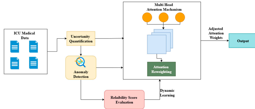
Figure 2. Design of the Robust Multi-Head Attention architecture, which contains the uncertainty quantification component, anomaly detection layer, and the attention reweighting components. The dynamically adjusting attention weights are generated by the mechanism using scores of the sample reliability calculated on the basis of training dynamics and gradient statistics.
