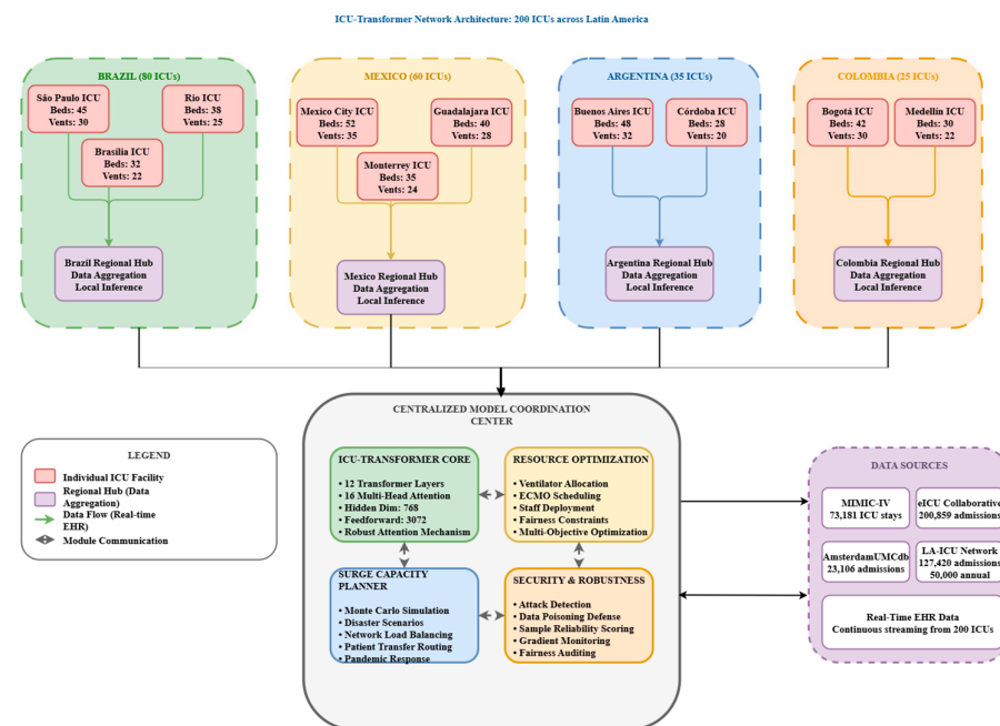
Figure 1. ICU-Transformer deployment network.
