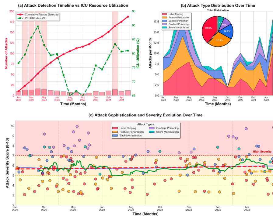
Figure 10. Attack progression over the 18-month deployment, showing a correlation between attack frequency and ICU resource utilization. Panel (a) highlights the attack detection timeline versus ICU utilization. Panel (b) shows the distribution of attack types over time. Panel (c) tracks attack sophistication and severity, with attack frequency correlating strongly with resource scarcity ( r = 0.67 , p < 0.001 ).
