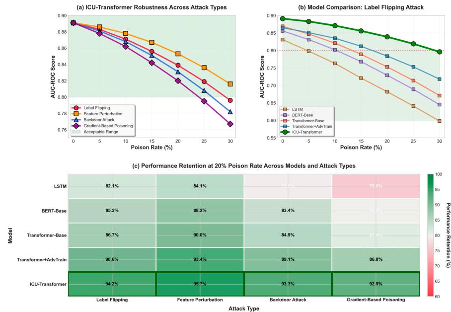
Figure 5. ICU-Transformer's robustness across various attack types at different poison rates. Panel (a) shows the model's AUC-ROC score degradation with increasing poison rates for different attacks: label flipping, feature perturbation, backdoor, and gradient-based poisoning. Panel (b) compares ICU-Transformer's performance specifically for the label flipping attack, with the AUC-ROC scores showing greater resilience than baseline models. Panel (c) illustrates performance retention at 20% poison rate across models and attack types, where ICU-Transformer maintains over 90% performance, outperforming other models.
