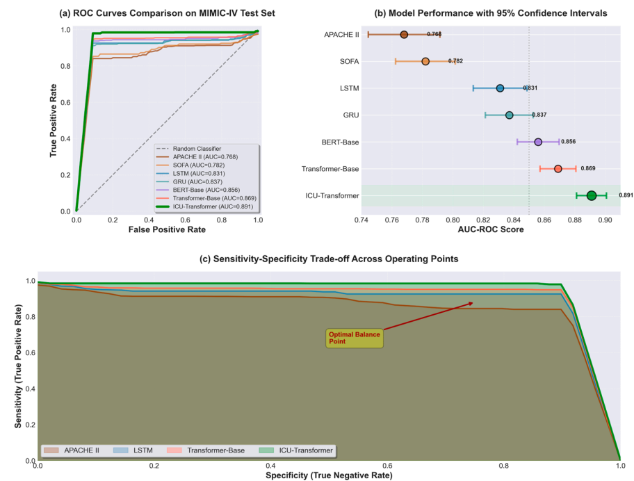
Figure 3. ROC curves of ICU-Transformer versus baseline models on the MIMIC-IV test set. The model achieves an AUC-ROC of 0.891, outperforming conventional transformer architectures and clinical scoring systems, demonstrating consistent high performance across all operating points. The figure also includes the 95% confidence intervals for the AUC-ROC scores, showing the statistical significance of the model's performance.
