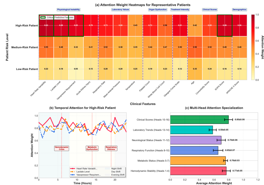
Figure 11. Attention weight heatmap showing the top three patients with varying mortality risks. Panel (a) displays how high-risk and low-risk patients focus on physiological instability indicators (e.g., heart rate variability, lactate level, vasopressor demand) and regular monitoring indicators, respectively. Panel (b) shows temporal attention for a high-risk patient, while Panel (c) illustrates multi-head attention specialization across different clinical features.
