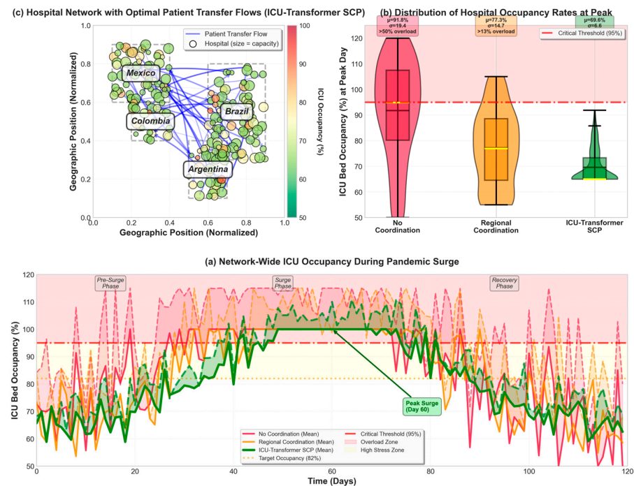
Figure 8. Surge capacity analysis showing ICU bed occupancy across the entire hospital network during a simulated pandemic surge. Panel (a) illustrates the network-wide ICU occupancy over time, with ICU-Transformer SCP optimizing the distribution of beds to prevent overcrowding in specific facilities. Panel (b) compares the distribution of hospital occupancy rates at peak occupancy, highlighting the advantages of regional coordination in ICU-Transformer SCP. Panel (c) shows the hospital network with optimal patient transfer flows, ensuring the most efficient and equitable allocation of ICU resources across different regions.
