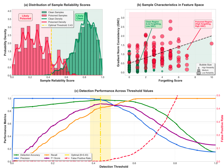
Figure 6. Sample rescored reliability scores calculated by ICU-Transformer for clean and poisoned samples in the MIMIC-IV training set under a 15% label flipping attack. Panel (a) shows the distribution of sample reliability scores, with clean and poisoned samples distinctly separated. Panel (b) illustrates sample characteristics in the feature space, where poisoned samples exhibit higher forgetting scores and gradient norm consistency (GNC) compared to clean samples. Panel (c)
