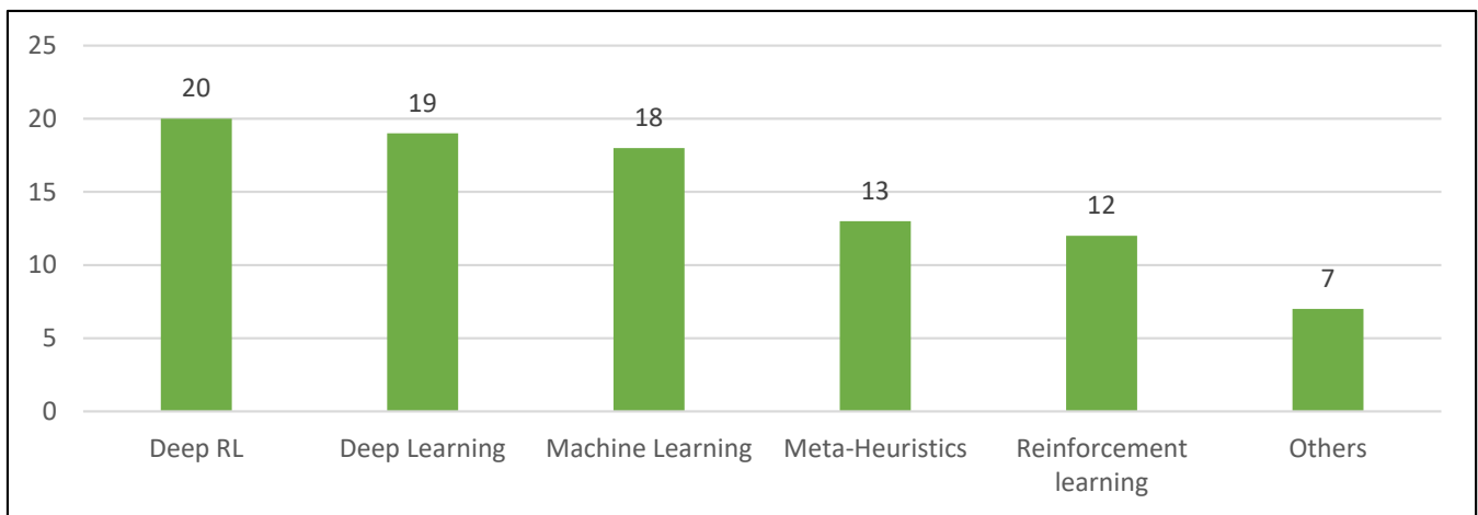
Figure 7. Method frequency.
