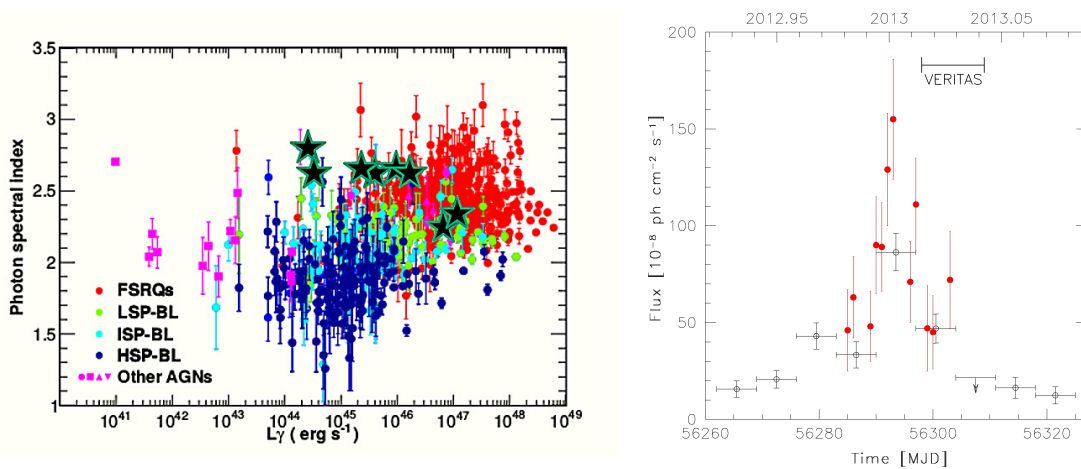
Figure 1. (Left panel): Photon index versus \gamma -ray luminosity of different types of Active Galactic Nuclei (AGN) included in the 3LAC. Black stars represent the values obtained over 7 years for narrow-line Seyfert 1 (NLSy1). Adapted from [20]; (Right panel): LAT light curve of PMN J0948+0022 in the 0.1–100 GeV energy range during 1 December 2012–31 January 2013 with 7-day time bins. Arrow refers to 2\text{-}\sigma upper limit. Upper limits are computed when TS < 10 . Red solid circles represent daily fluxes reported for the periods of high activity. The horizontal line indicates the period of the VERITAS observation. Adapted from [13].
