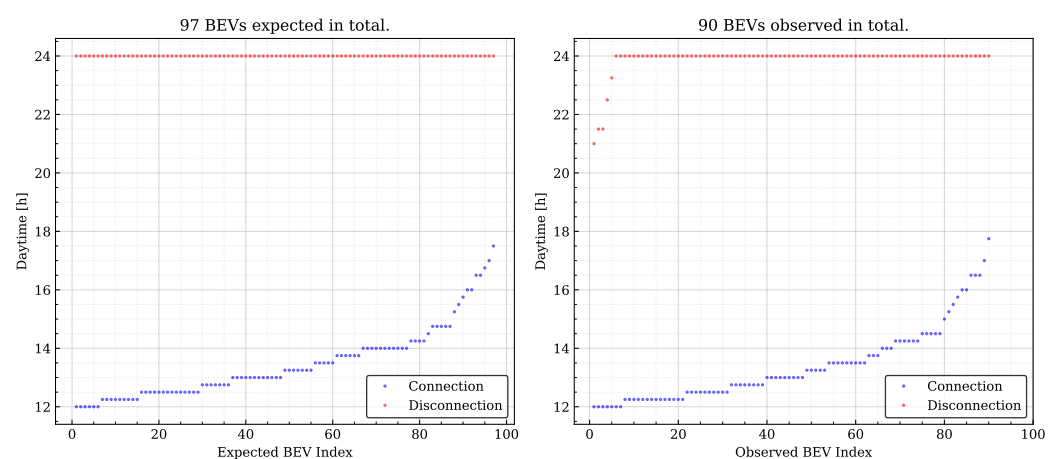
Figure A5. Expected and observed BEV population for non-mixed-discharging BEVs.
