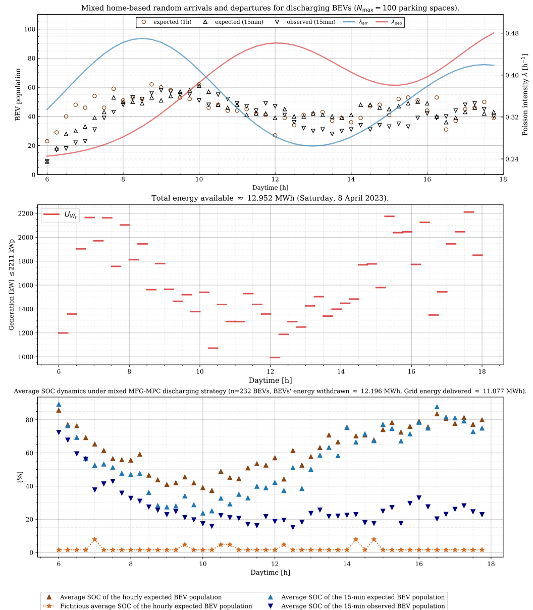
Figure 8. Vehicle-to-grid MFPC mixed-discharging results: (top) —expected and observed BEV population using mixed home-based Poisson intensities; (middle) —aggregate power (generation); (bottom) —average SOC dynamics.
