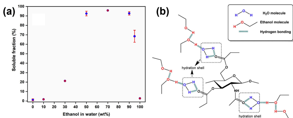
Figure 4. (a) Solubility profile of chitin propionate in ethanol/water binary solvent systems with varying ethanol concentrations; (b) schematic illustration of possible hydrogen bonding interactions between chitin propionate repeating units, water molecules, and ethanol molecules. Reproduced with permission from [35].
