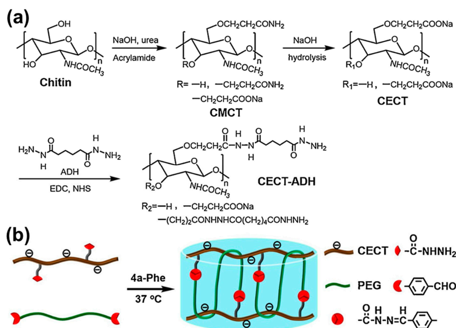
Figure 7. Fabrication of CECT-ADH and CECT-ADH/PEG-DA hydrogels. (a) Synthesis pathway of CECT-ADH; (b) Schematic representation of CECT-ADH/PEG-DA hydrogel formation through dynamic acylhydrazone crosslinking interactions. Reproduced with permission from [15].
