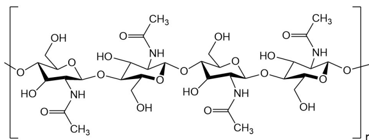
Figure 1. Chemical structure of chitin poly(N-acetyl- \beta -d-glucosamine).
