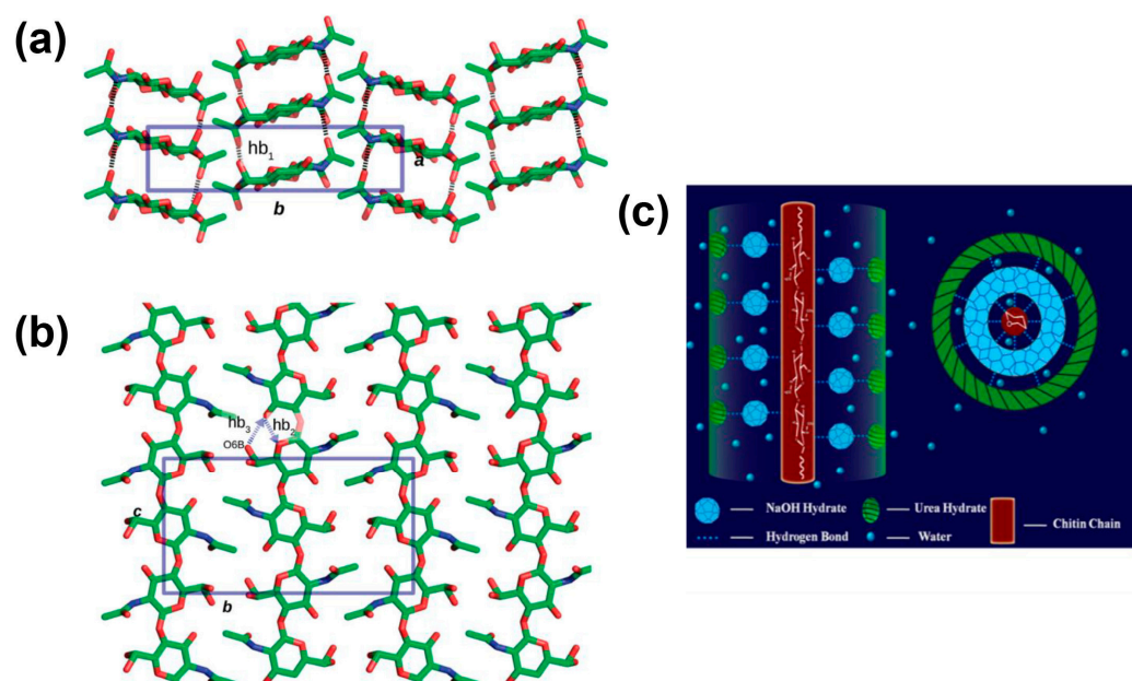
Figure 2. Crystalline configurations of \alpha -chitin and \beta -chitin. (a) Top-to-bottom vertical views along the ab- and (b) bc- planes of the \alpha -chitin structure at 100 K (Reproduced with permission from [26]). (c) A structural model of chitin complex chain in an aqueous NaOH/urea system (reproduced with permission from [27]).
