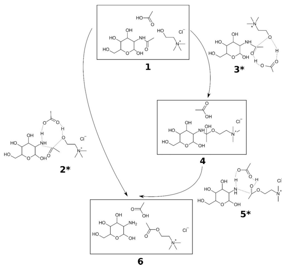
Figure 5. Molecular structures, including intermediates and transition states (denoted by asterisks), involved in the deacetylation of GlcNAc using [Ch]Cl:AA. The reaction may follow either a single-step pathway (1,2*,6) or a two-step pathway (1,3*,4,5*,6). A comparable reaction mechanism is observed with [Ch]Cl:OA and [Ch]Cl:MA systems. Reproduced with permission from [37].
