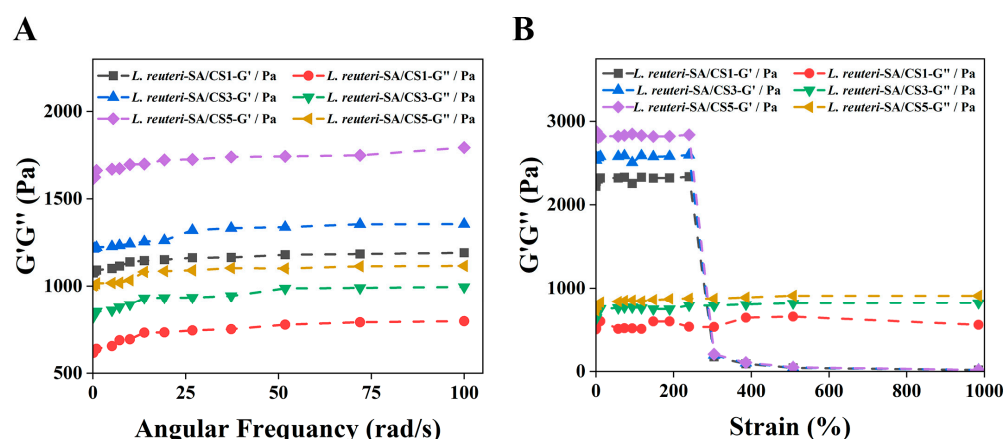
Figure 5. Rheological properties of L. reuteri -SA/CS1-5 hydrogels. (A) Storage modulus ( G' ) and loss modulus ( G'' ) as functions of angular frequency; (B) Storage modulus ( G' ) and loss modulus ( G'' ) as functions of strain.
