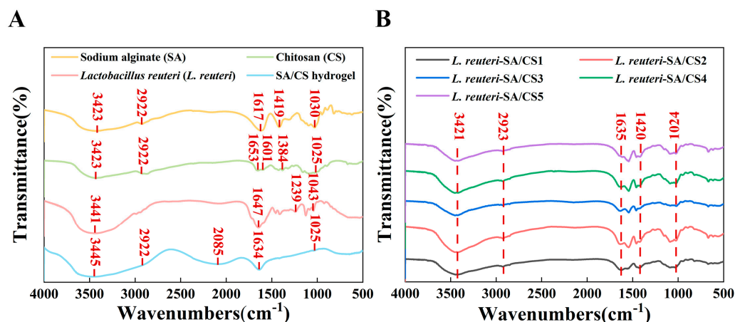
Figure 4. Fourier transform infrared (FTIR) spectra of the individual components and probiotic-loaded SA/CS hydrogels. (A) Sodium alginate (SA), chitosan (CS), Lactobacillus reuteri (L. reuteri), and the SA/CS hydrogel. (B) L. reuteri -SA/CS1-5 hydrogels.
