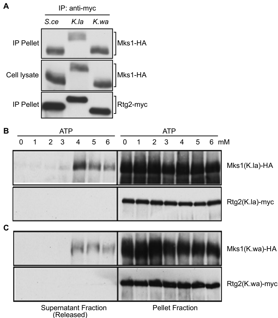
Figure 5. ATP releases Mks1 from Rtg2. (A) Rtg2 and Mks1 homologs from K. lactis and K. waltii form a complex. rtg2Δ mks1Δ double mutant cells (ZLY145) expressing pairs of epitope-tagged Rtg2 and Mks1 from indicated fungal species were analyzed for interaction between Rtg2 and Mks1 using co-immunoprecipitation. Rtg2-myc was precipitated using anti-myc anti-body. Rtg2-myc and Mks1-HA were detected by immunoblotting. (B and C) ATP at physiological concentrations has an all-or-none effect on releasing the Mks1 homolog from the Rtg2 homolog from K. lactis (B) and K. waltii (C). The effect of ATP on the release of Mks1 from immunopurified Rtg2-Mks1 complexes was analyzed as described for Figure 2.
