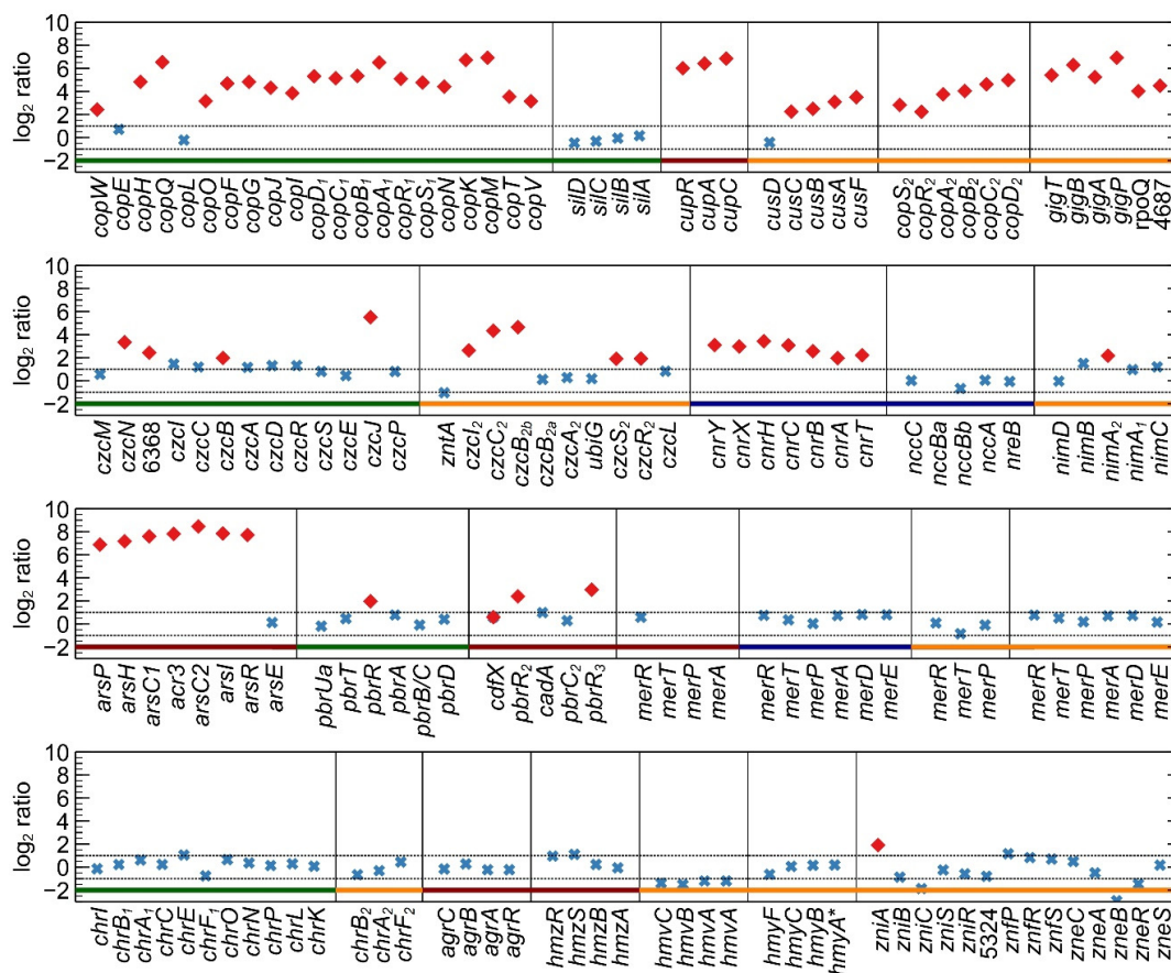
Figure 1. Differential gene expression of metal resistance genes from C. metallidurans CH34 exposed for 10 min to 400 \mu\text{M} \text{Cu}^{2+} . Significant (red diamond; p < 0.05 ) and non-significant (blue cross) \log_2 ratios are shown for known metal resistance genes located on the chromosome (red line under graph), chromid (orange), pMOL28 (blue), and pMOL30 (green). Dotted lines correspond to -1 and 1 , respectively.
