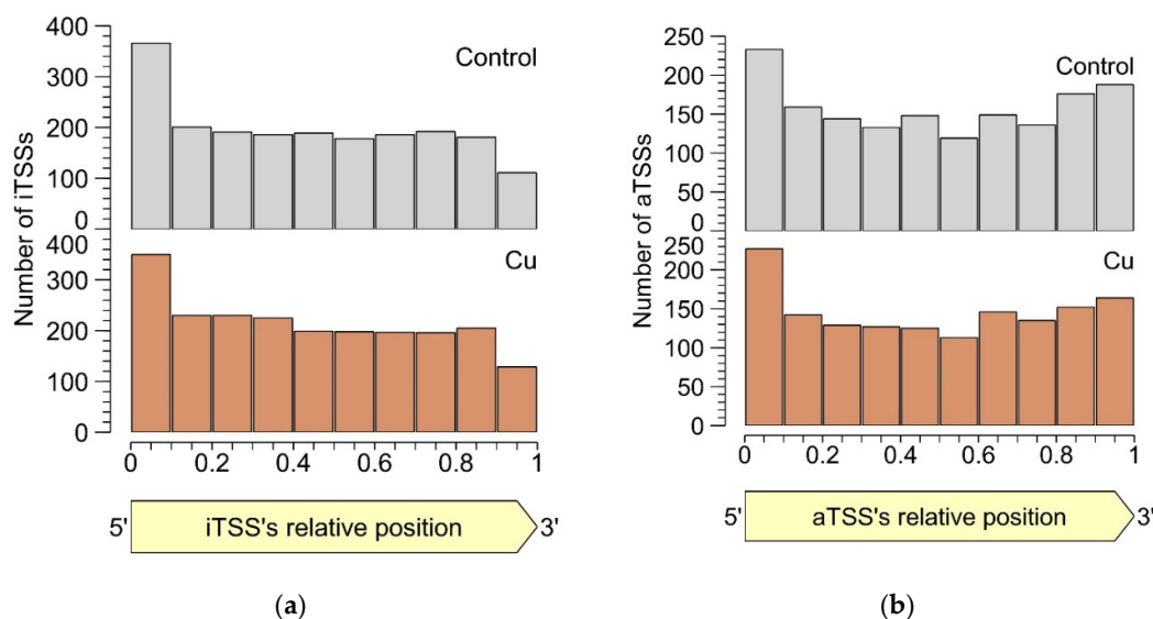
Figure 4. Percentile-wise distribution of iTSSs (a) and aTSSs (b) positions relative to the cognate CDS.
