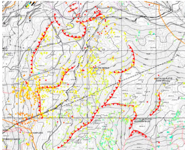
Figure 7. The deep earthflow in Cervinia.
