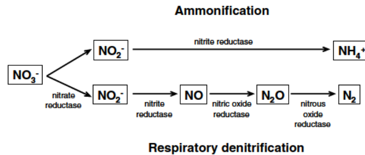
Figure 7. Nitrate and nitrite reduction [48].
