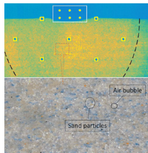
Figure 6. Centrifuge model layout (a) and colour of fully saturated soil (green) (b) and partially saturated soil (yellow) (c), where brighter yellows indicate lower degrees of saturation (modified after Zeybek and Madabhushi [43]).
