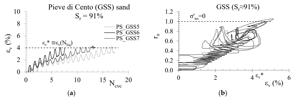
Figure 15. Volumetric strain with the number of cycles (a) and r_u with \varepsilon_v (b) (modified after [31]).
