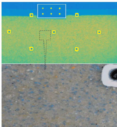
Figure 6. Centrifuge model layout (a) and colour of fully saturated soil (green) (b) and partially saturated soil (yellow) (c), where brighter yellows indicate lower degrees of saturation (modified after Zeybek and Madabhushi [43]).
