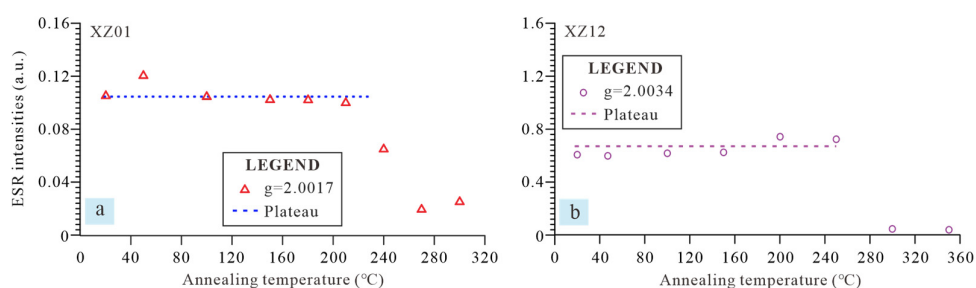
Figure 8. Thermal stabilities of the paramagnetic center at g = 2.0017 of XZ01 (a) and at g = 2.0034 of XZ12 (b).
