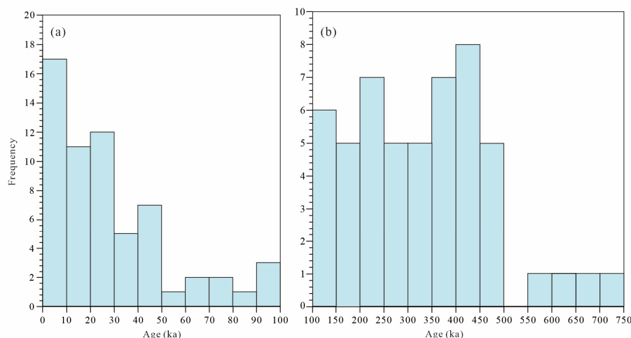
Figure 10. Histogram showing distributions of silica sinter and travertine ages in 10 kyr step width from 100 kyr (a) and in 50 kyr step width from 750 to 100 kyr (b). Different bin widths were chosen to optimize display for each interval.
