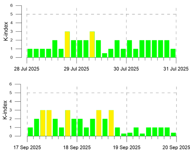
Figure 2. Variations in the geomagnetic K-index before and during the Kamchatka earthquakes that occurred in July and September 2025, based on data from the geomagnetic observatory “Alma-Ata”.
