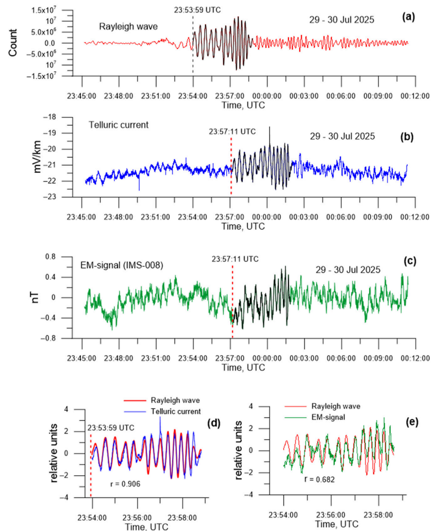
Figure 6. Coseismic response of the telluric current and electromagnetic ULF signals to the propagation of Rayleigh wave generated by the M8.8 earthquake: (a) seismogram of the vertical (Z) component of the Rayleigh wave; (b) telluric current; (c) electromagnetic ULF signal. The wave packets are highlighted in black. Results of the cross-correlation analysis obtained by aligning the telluric current records (d) and EM signal records (e) with the seismic wave in the zone of maximum correlation using a time shift of \Delta t = 191.7 s. Vertical dashed lines indicate the arrival times of the wave trains for which the maximum cross-correlation coefficient was obtained.
