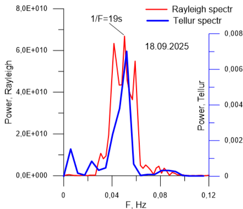
Figure 10. Comparison of wave train power spectra for telluric current variations (blue) and the Rayleigh wave (red), generated by the 18 September 2025 earthquake ( M7.8 ).
