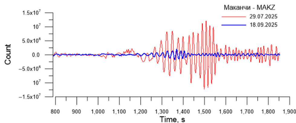
Figure 7. Comparison of the waveforms and amplitudes of the Rayleigh waves generated by the 29 July 2025 M8.8 earthquake and the 18 September 2025 M7.8 earthquake. The seismograms were aligned along the time axis for ease of comparison.
