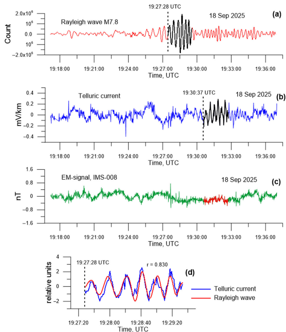
Figure 8. Coseismic response of the telluric current to the Rayleigh wave propagation generated by the M7.8 earthquake: (a) seismogram of the vertical (Z) component of the Rayleigh wave; (b) telluric current variations; (c) ULF electromagnetic (EM) signal. The wave packets are highlighted in black. (d) Result of the cross-correlation analysis obtained by aligning the telluric current record with the seismic wave in the zone of maximum correlation using a time shift of \Delta t = 191.7 s. Vertical dashed lines indicate the arrival times of the wave packets for which the maximum cross-correlation coefficient was obtained.
