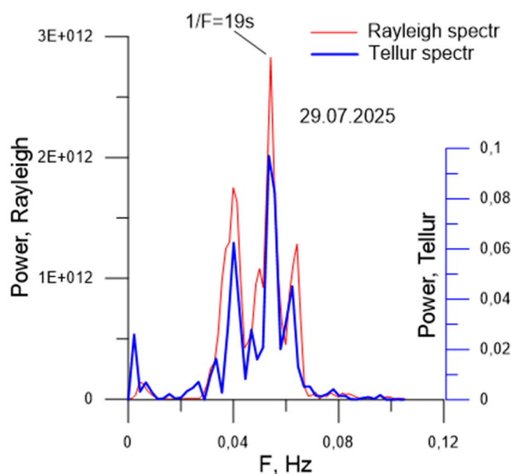
Figure 9. A comparison of the wave train power spectra for telluric current variations (blue) and Rayleigh wave oscillations (red) generated by the M8.8 Kamchatka earthquake (29 July 2025).
