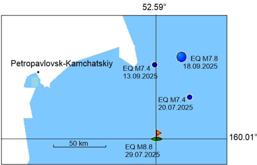
Figure 3. Spatial distribution of the epicenters of Kamchatka earthquakes with magnitudes M7.4–7.8 (blue circles) and the epicenter of the M8.8 earthquake (red flag) that occurred during the summer–autumn period of 2025.
