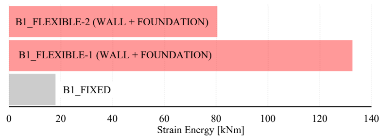
Figure 32. The dissipated energy of the wall (+ foundation) for nonlinear dynamic loading of Building 1 models.
