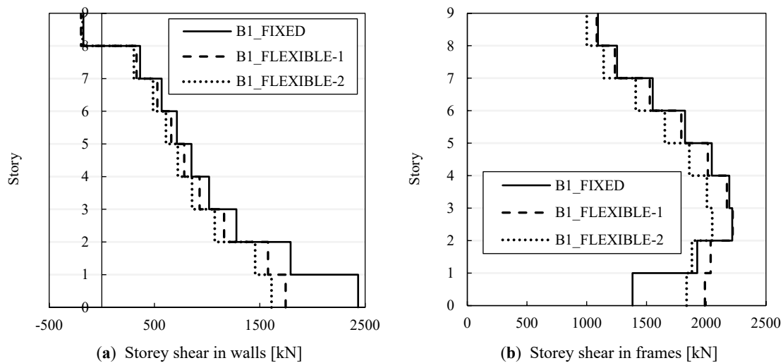
Figure 8. Contribution of walls (a) and frames (b) in resisting shear forces in Building 1 models.
