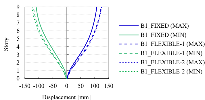
Figure 23. Displacement shapes of Building 1 models.
