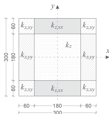
Figure 4. Spring zones in footing F1.
