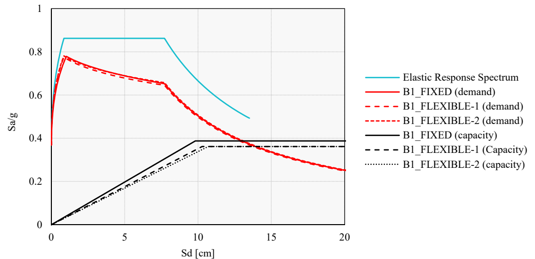
Figure 20. Performance assessment of Building 1 models.
