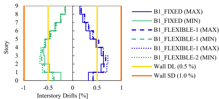
Figure 24. Interstory drift ratios for Building 1 models.
