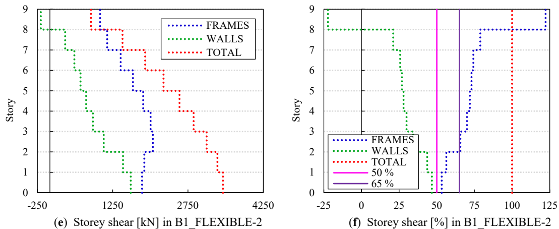
Figure 9. Wall and frame contributions to resisting shear forces on B1_FIXED model (a,b), B1_FLEXIBLE-1 model (c,d), and B1_FLEXIBLE-2 model (e,f).
