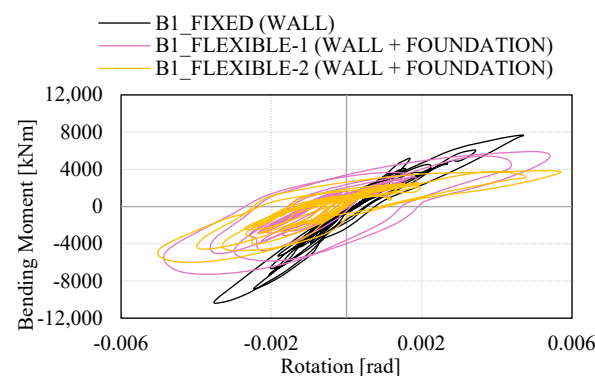
Figure 31. Hysteresis loop curves for section a-a at the wall in Building 1 models. Distribution of strain energy between the wall and the foundation in: (a) B1_FLEXIBLE-1 model and (b) B1_FLEXIBLE-2 model.
