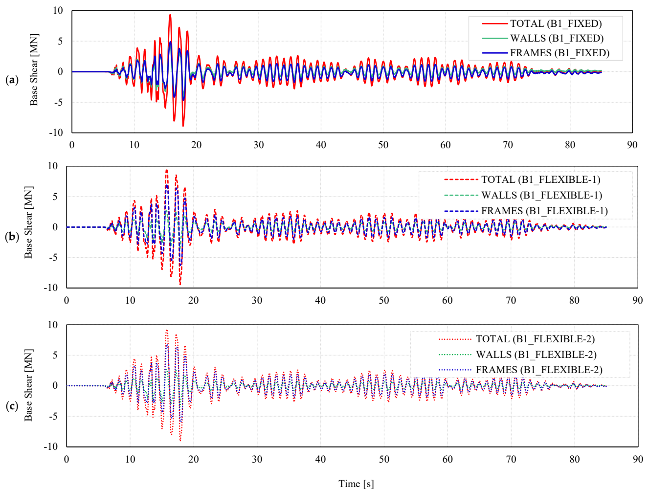
Figure 26. Base shear time histories and their distribution among the walls and frames for B1_FIXED (a), B1_FLEXIBLE-1 (b) and B1_FLEXIBLE-2 (c) models.
