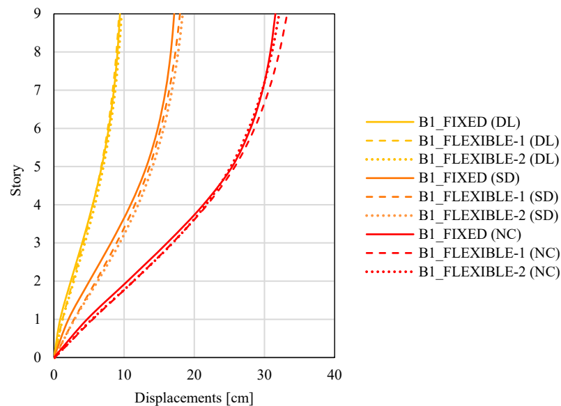
Figure 11. Displacement shapes of Building 1 models for the three limit states.
