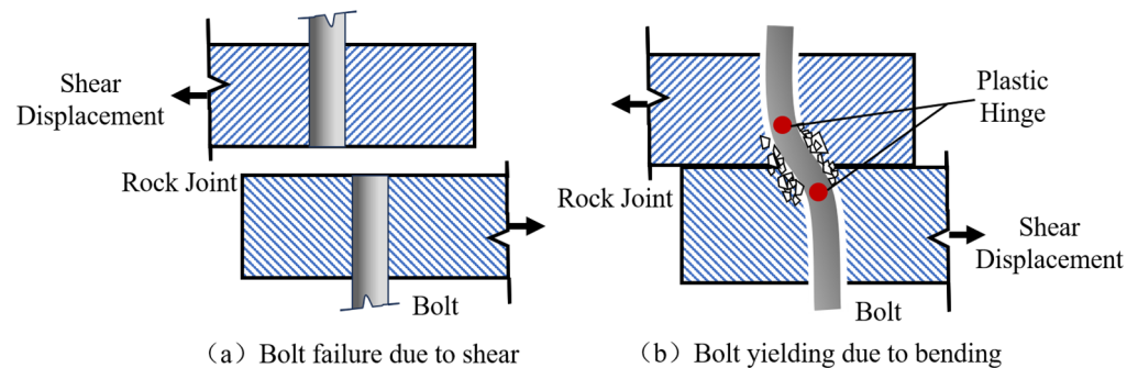
Figure 3. Failure modes of bolts at rock joints: (a) shear failure, where the bolt is fractured across the rock joints; (b) bending yield, where a plastic hinge is formed in the bolt due to bending deformation.
