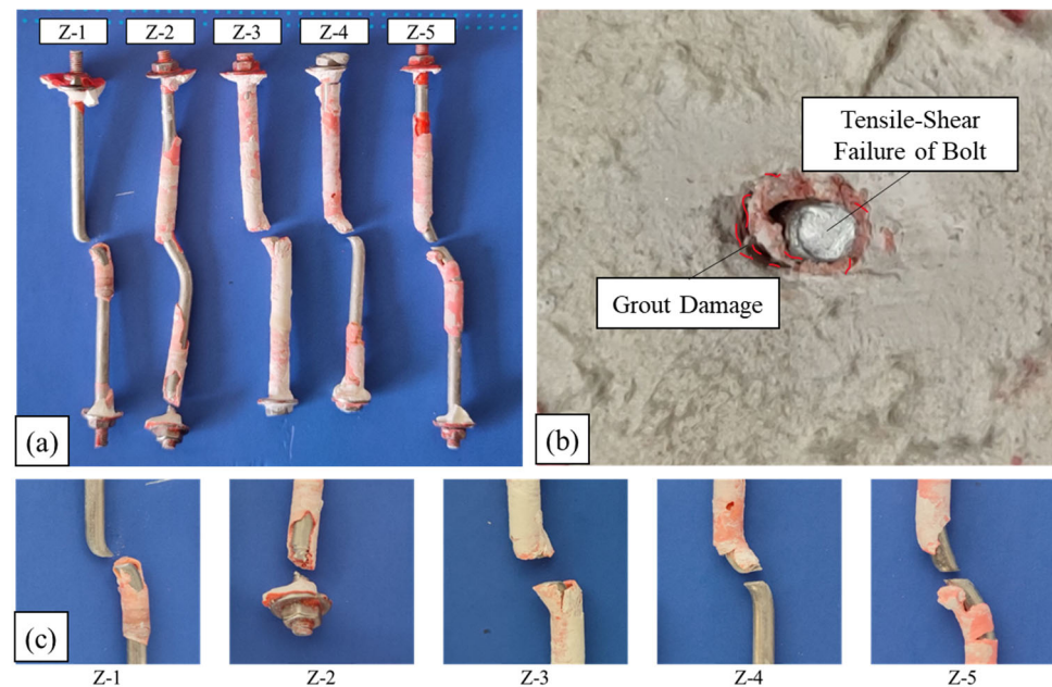
Figure 7. Failure characteristics of fully grouted bolts at rock joints: (a) overall failure modes of bolts in the fully anchored condition; (b) localized tensile-shear fracture of the bolt at the rock joints; (c) detailed views of the bolt fracture morphology.
