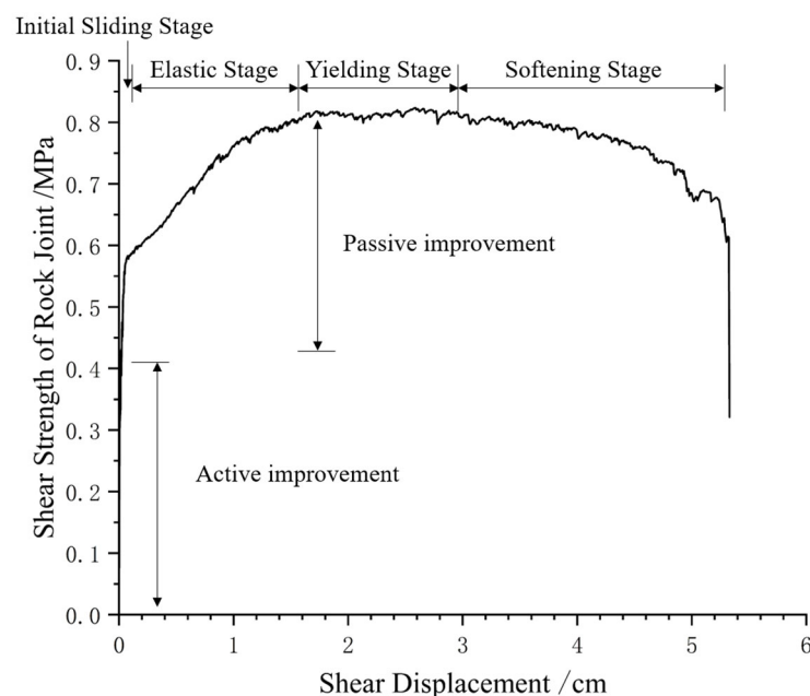
Figure 1. Shear strength variation in bolted rock joints.
