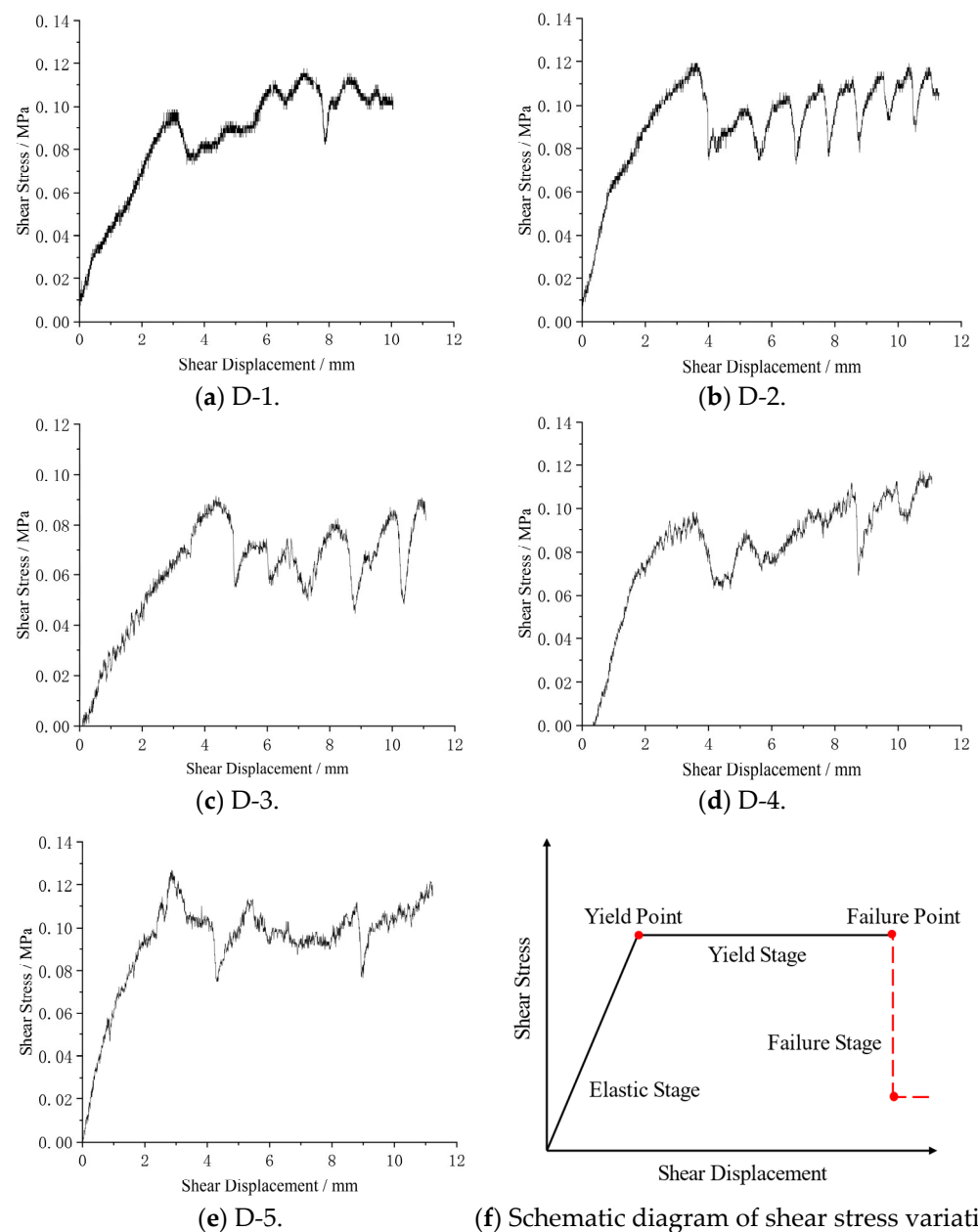
Figure 8. The change curve of shear stress of a rock joint under end-anchoring. Note: In (f), the solid line represents experimentally obtained data; the dashed line indicates the inferred failure stage extrapolated from numerical simulations, as the physical test was terminated at the 12 mm displacement limit before bolt fracture occurred.
