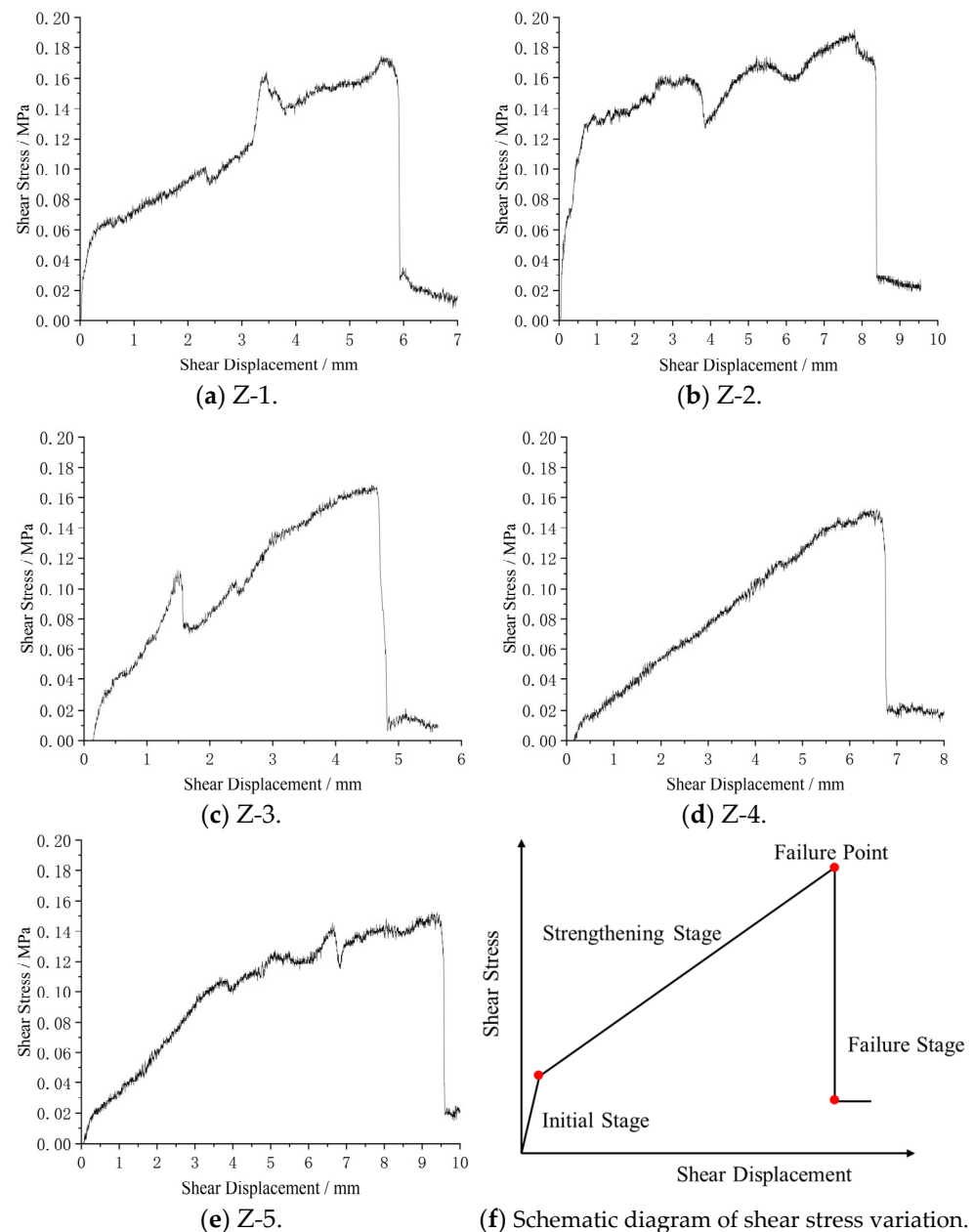
Figure 6. The variation curve of shear stress of the rock joint under a full-anchor condition.
