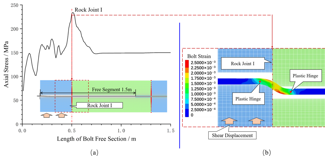
Figure 15. Mechanical response of the bolt under shear loading. (a) Axial stress distribution along the free section. (b) Axial strain distribution indicating the development of plastic hinges at the joint interface.
