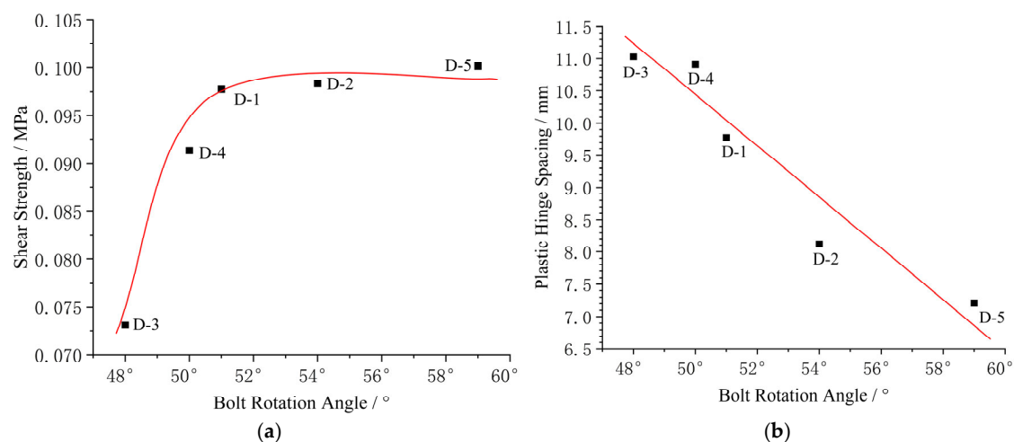
Figure 11. Relationship between bolt rotation angle and mechanical properties: (a) shear strength, and (b) plastic hinge spacing.
