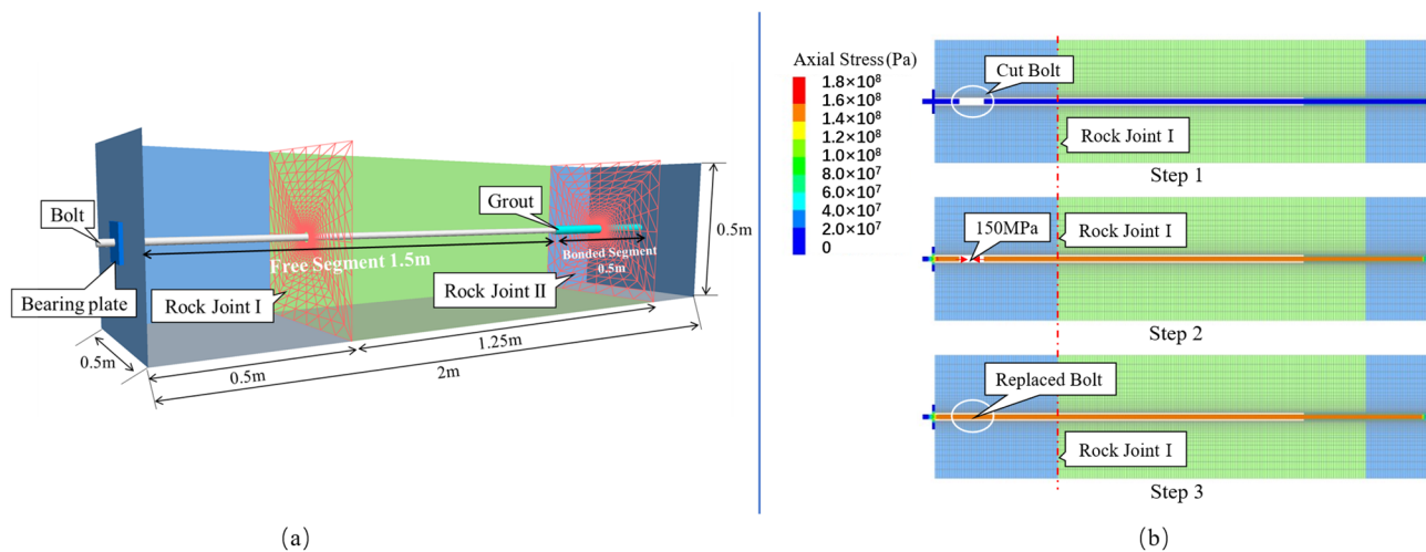
Figure 13. Numerical model for the bolted rock mass with two rock joints and steps for applying prestress. (a) Model setup. (b) Prestress application procedure (Steps 1–3).
