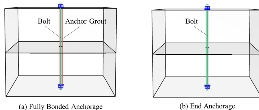
Figure 4. Schematic diagram of specimens with different anchoring conditions.
