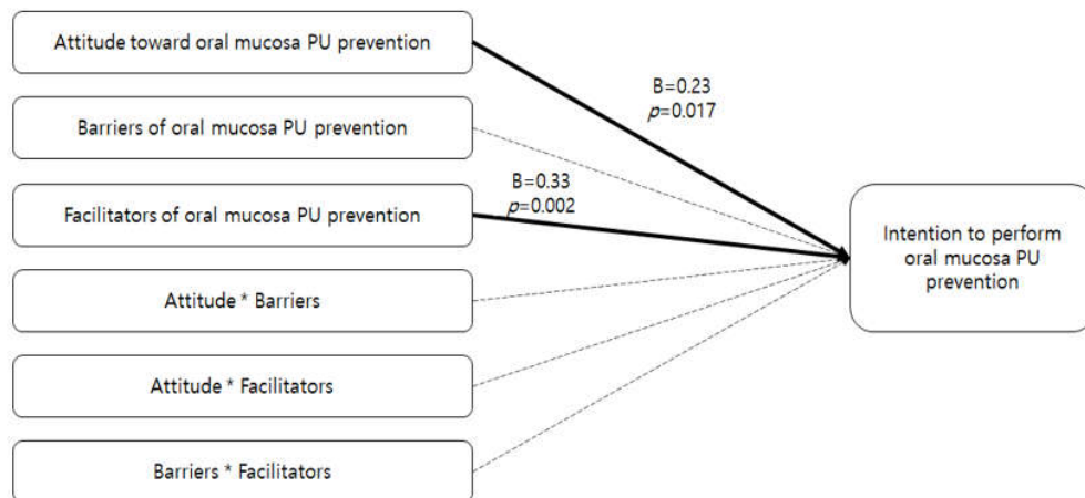
Figure 1. Diagram for results of multiple regression.
