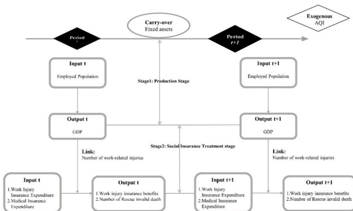
Figure 1. Model framework.
