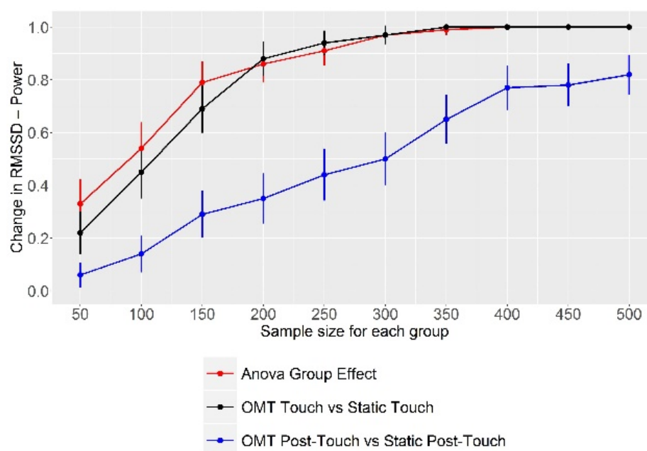
Figure 1. Power analysis via Monte Carlo simulation. The x-axis shows the sample size for each group: therefore, the total sample size for each point equals two times its corresponding x-axis value (e.g., a value of 100 on the x-axis corresponds to a total sample size of 200). For every sample size evaluated, the graph reports the power \beta for detecting a statistically significant change in RMSSD value: as revealed by the ANOVA group main effect; between the Dynamic Touch group and the Static Touch group during the intervention; between the Dynamic Touch group and the Static Touch group after the intervention. Abbreviations: RMSSD, root mean squared successive differences.
