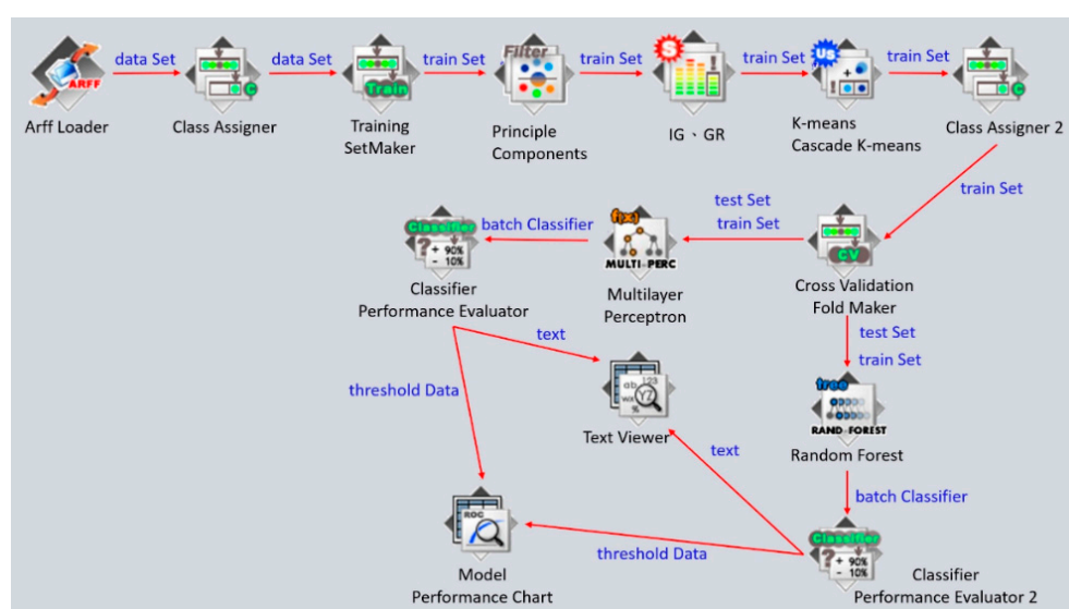
Figure 3. Clustering and classification validation with WEKA.
