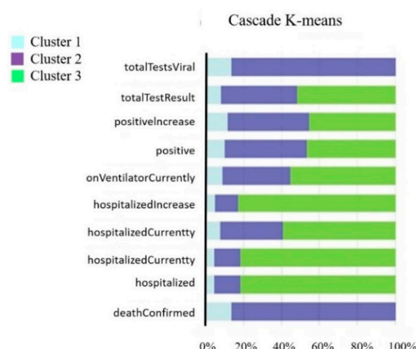
Figure 4. Cluster characteristics.
