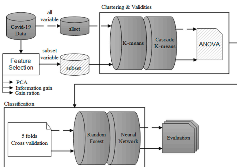
Figure 1. Clustering analysis and classifications scenario.
