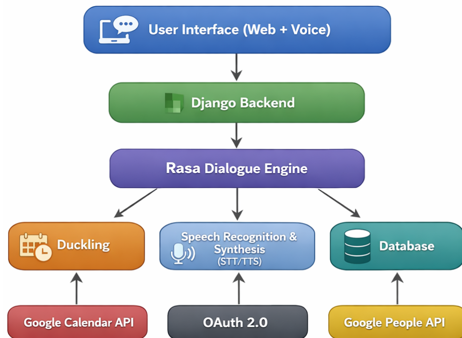
Figure 1. System architecture of the UjaBienestar multimodal conversational platform.
