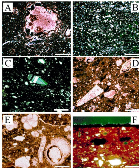
Figure 8. (A) RC269: large clot of microcrystalline calcite (micrite), likely formed by thermal decomposition of a calcareous bioclast or lithic fragment (XPL, scale bar = 0.5 mm); (B) RC268: very-fine-to-fine aplastic inclusions of quartz (dominant) and subordinate feldspars, homogeneously dispersed in an optically inactive groundmass (XPL, scale bar = 0.1 mm); (C) RC273: details of a polysynthetically twinned plagioclase grain, ~0.15 mm in size (XPL, scale bar = 0.5 mm); (D) RC271: coarse-to-medium-sand-sized aplastic inclusions represented by bioclasts and calcarenite fragments (XPL, scale bar = 0.5 mm); (E) RC271: remains of planktonic and benthic foraminifera (PPL, scale bar = 0.1 mm); (F) RC276: details of the black paint layer, regular and only 0.01–0.02 mm thick (XPL, scale bar = 0.1 mm).
