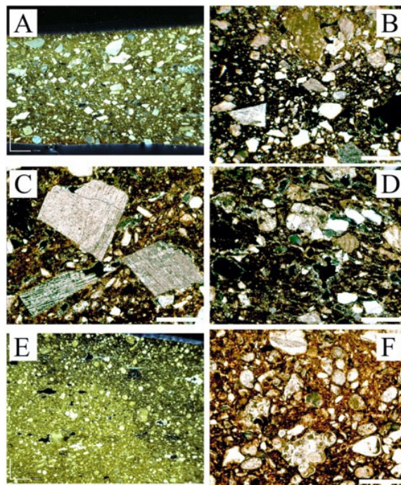
Figure 10. (A) RC288: general view showing crushed crystalline calcite inclusions homogeneously dispersed within the groundmass (Dinolite digital polarization; scale bar = 1 mm); (B) RC297: aplastic fraction predominantly composed of crushed spathic calcite, with minor quartz and pelagic limestone fragments (XPL; scale bar = 0.5 mm); (C) RC291: polysynthetically twinned calcite grains with euhedral habit, deriving from characteristic rhombohedral cleavage, measuring 0.3–0.4 mm (XPL; scale bar = 0.2 mm); (D) RC289: remains of bioclasts and lower Miocene macroforaminifera together with quartz grains (XPL; scale bar = 0.2 mm); (E) RC295: middle Miocene bioclasts prevailing over quartz grains (XPL; scale bar = 1 mm); (F) RC295: middle Miocene bioclasts prevailing over quartz grains, with evidence of external burnishing (Dinolite digital polarization; scale bar = 1 mm);
