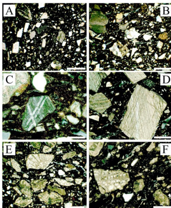
Figure 9. (A) RC283: general view showing crushed crystalline calcite inclusions homogeneously dispersed in the groundmass (XPL, scale bar = 0.5 mm); (B) RC282: finest aplastic fraction composed mainly of quartz and feldspars (XPL, scale bar = 0.5 mm); (C) RC278: polysynthetically twinned calcite grain, ~0.25 mm in size (XPL, scale bar = 0.1 mm); (D) RC281: lamellar twinning and cleavage traces in euohedral calcite crystals (XPL, scale bar = 0.2 mm); (E) RC280: remains of benthic foraminifera (XPL, scale bar = 0.5 mm); (F) RC280: detail of bioclasts and coarse silt-sized quartz grains (XPL, scale bar = 0.2 mm).
