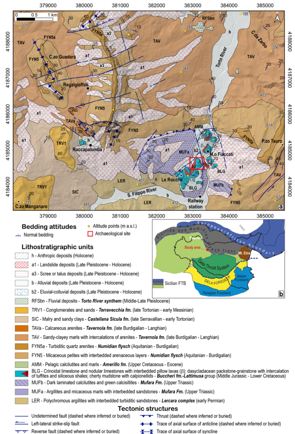
Figure 6. Geological sketch map of the study area (a), modified from [11,12]. New field surveys in the southern sector completed the geological and structural mapping and provided bedding-attitude measurements. The map was produced in QGIS 3.16 using a 5 m resolution DEM as topographic base. (b) Structural map of the main elements of the Sicilian collisional complex (modified from [8,9]).
