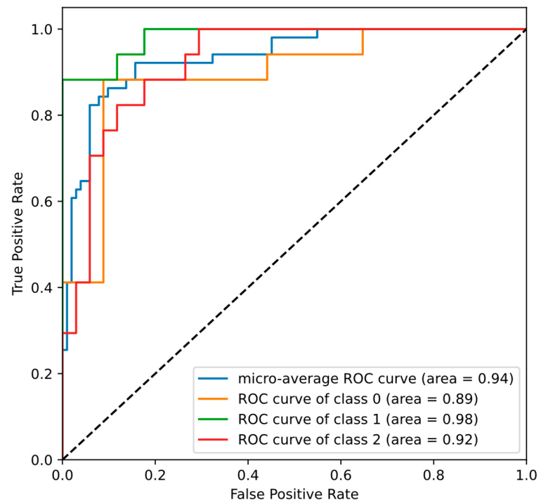
Figure 12. ROC curves and ROC-AUC values for the 3D-CNN architecture based on the GoogLeNet classifier model: Unbruised (Class 0), Bruised-1 (Class 1), and Bruised-2 (Class 2), and unripe and ripe fruit cases.
