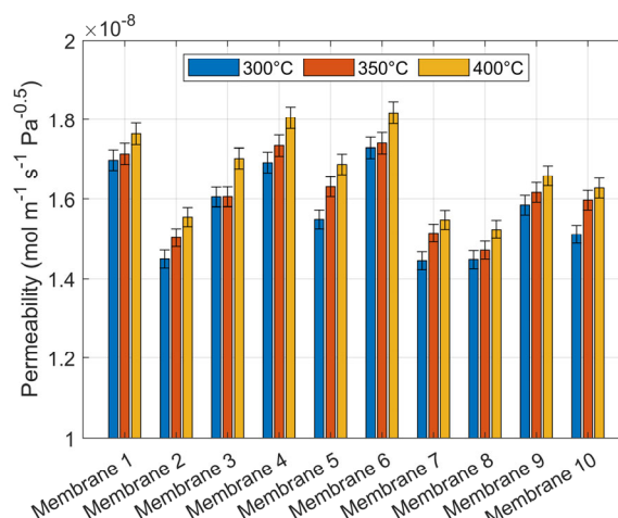
Figure 4. Permeability of the membranes as a function of temperature.
