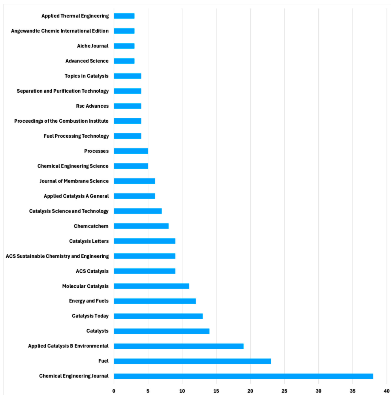
Figure 9. Distribution of analysed publications across journals.
