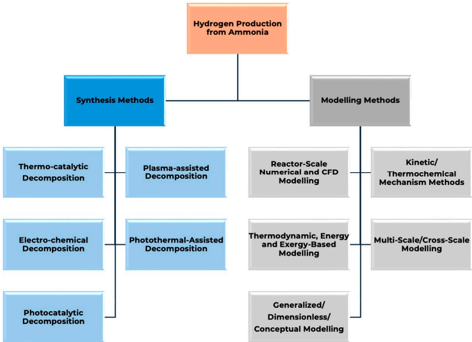
Figure 3. Flowchart of the synthesis and modelling classifications.
