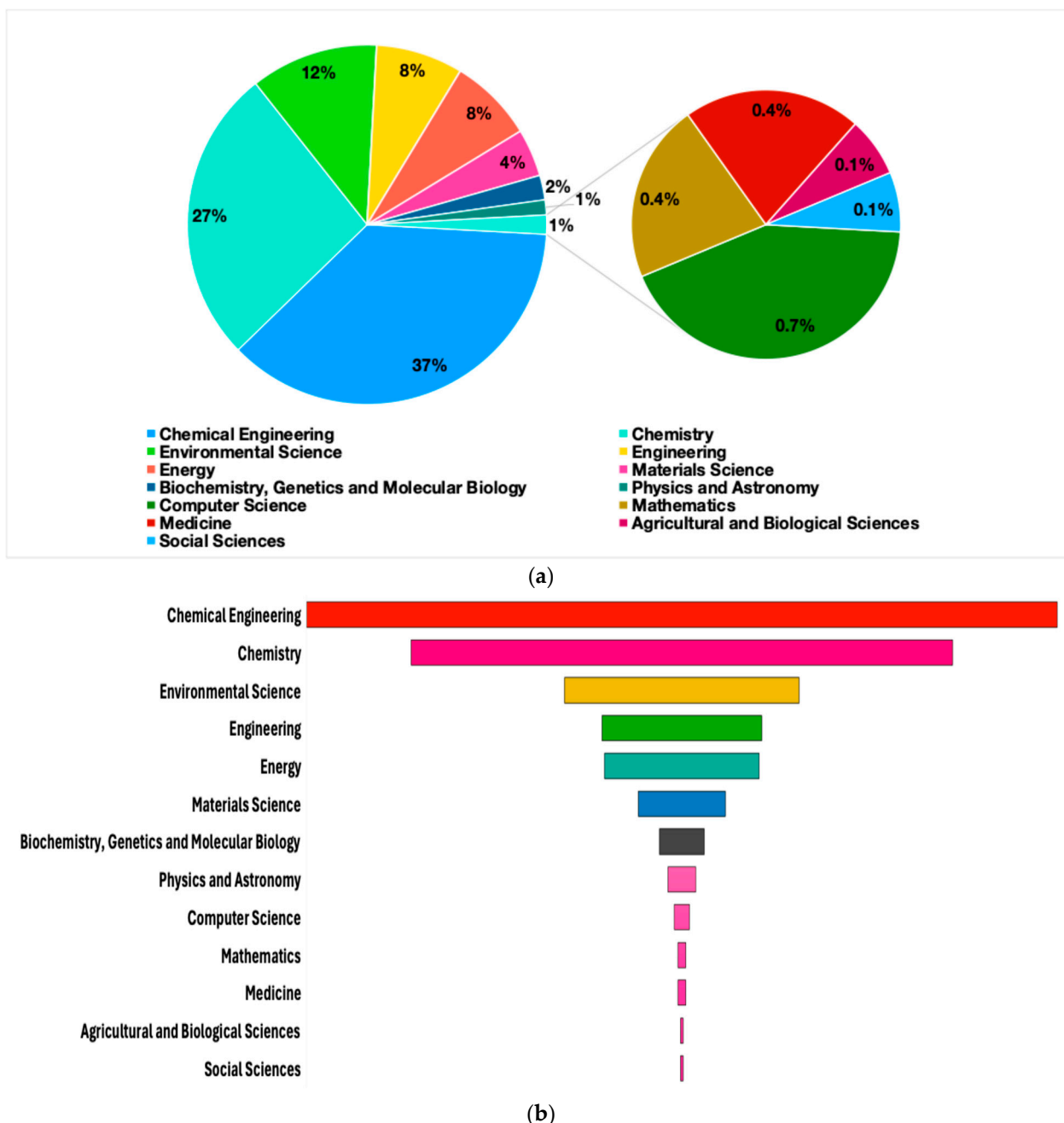
Figure 8. Subject-area distribution of the analysed publications presented as (a) a pie chart and (b) a funnel chart, illustrating the relative contribution and hierarchical dominance of disciplines involved in ammonia decomposition modelling research.
