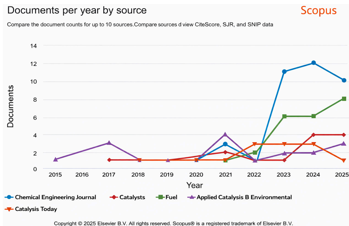
Figure 5. Annual distribution of modelling and simulation studies on ammonia decomposition for hydrogen production across major journals included in the final dataset.
