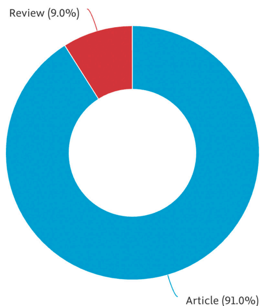
Figure 6. Document-type distribution of the analysed publications.
