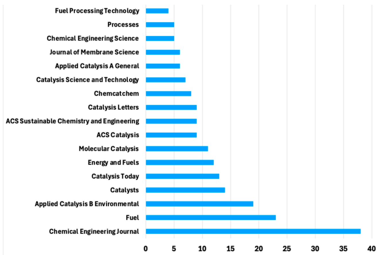
Figure 7. Distribution of analysed publications by subject area.
