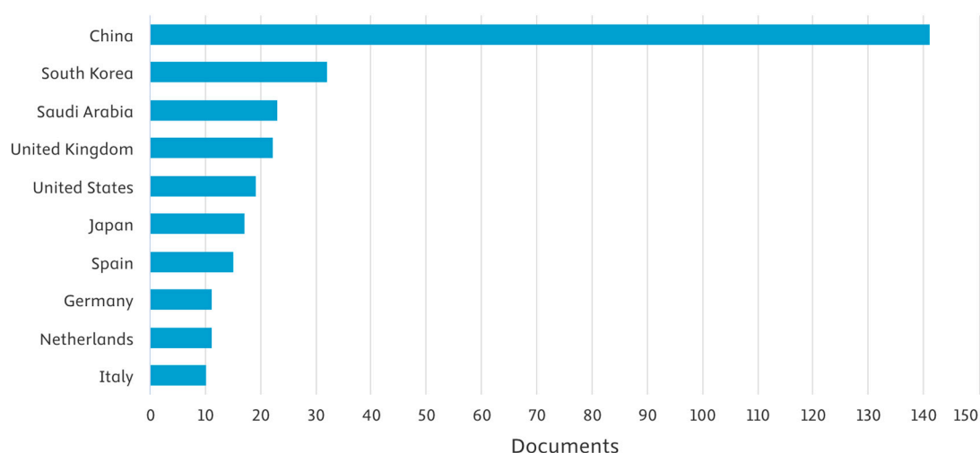
Figure 11. Distribution of analysed publications by country based on author affiliation.
