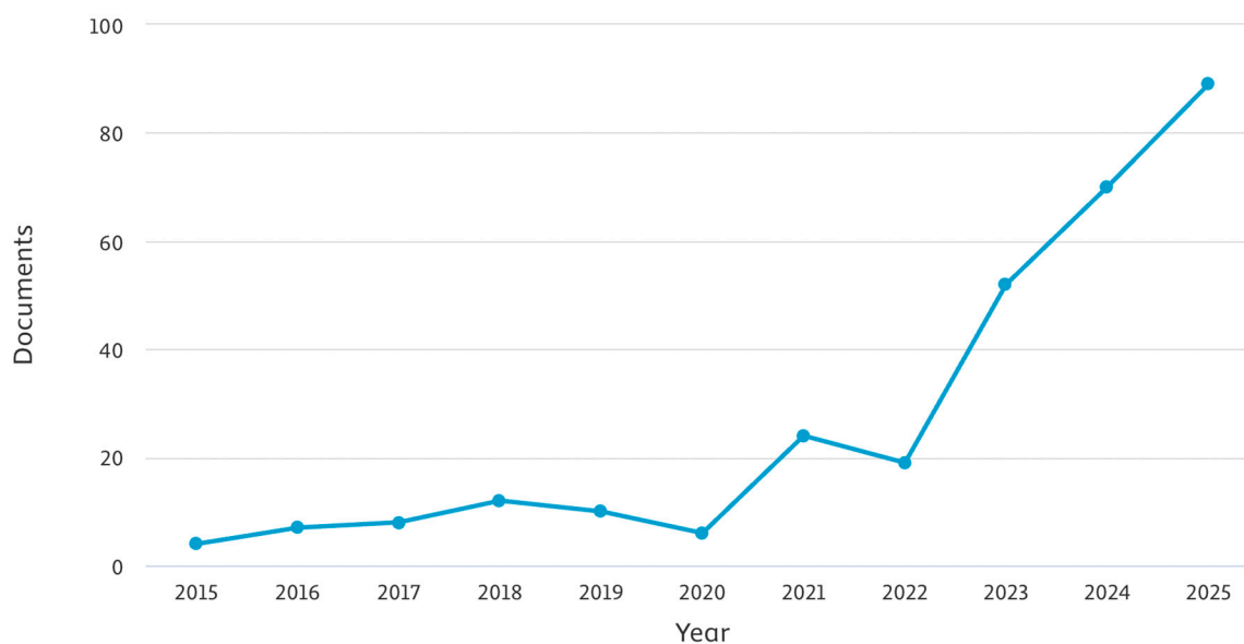
Figure 4. Annual distribution of modelling and simulation studies on ammonia decomposition for hydrogen production is included in the final dataset.
