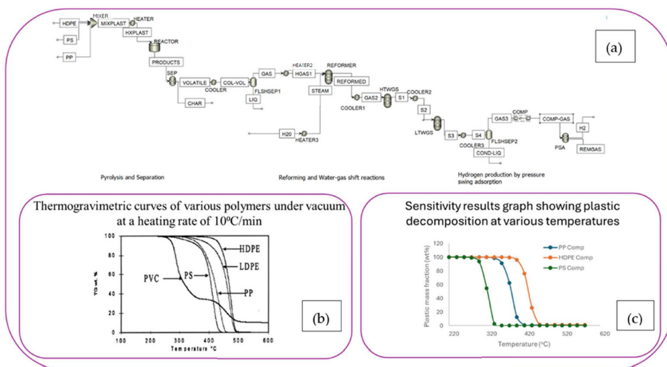
Figure 1. (a) Process flow diagram of the pyrolysis–reforming system. (b) Thermogravimetric curves of polymers obtained under vacuum at a heating rate of 10\text{ }^{\circ}\text{C min}^{-1} [101]. (c) Sensitivity analysis showing order of thermal stability of plastic decomposition, validating the thermogravimetric behaviour observed in (b).
