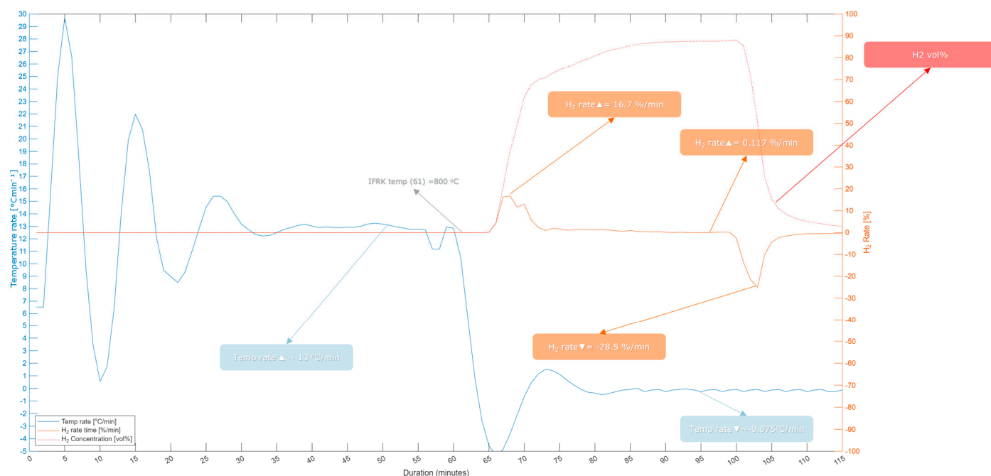
Figure 14. Temperature-rate profile, outlet-H 2 concentration and calculated H 2 signal slopes for Reduction #1, performed with the −1 mm laterite fraction at 800 °C.
