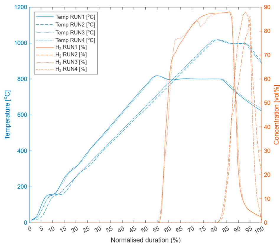
Figure 18. Normalised kiln-temperature and outlet-H 2 concentration profiles for the four laterite reduction experiments.
