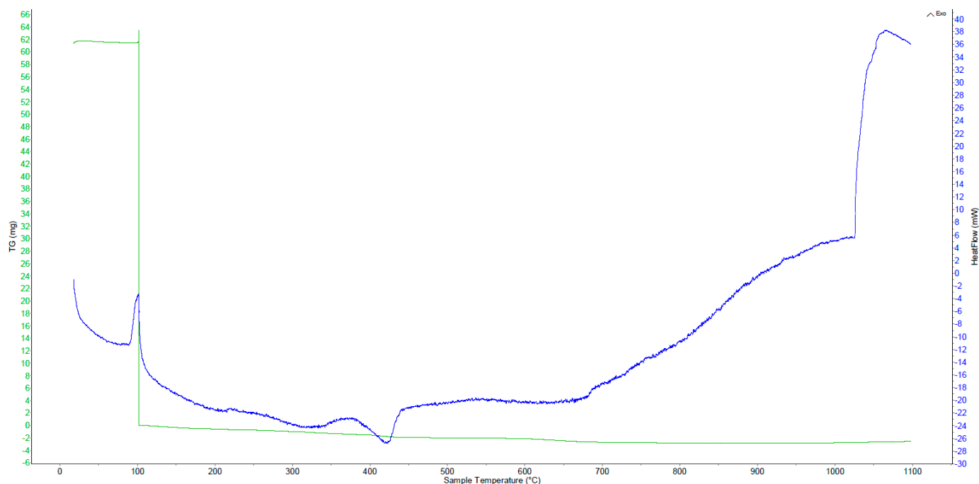
Figure 11. TG–DTA curves of magnesite before and after IFRK calcination. Green lines refer to TG curves, blue lines refer to DTA curves.
