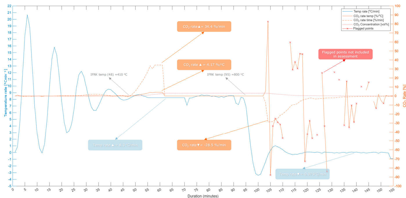
Figure 7. Temperature-rate profile, outlet-CO 2 concentration and calculated CO 2 signal slopes for the 800 °C magnesite calcination experiment.
