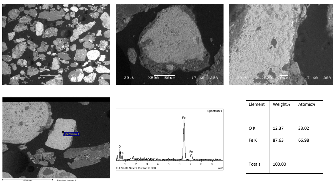
Figure 21. Representative SEM images and local EDS analyses of the −1 mm laterite fraction after hydrogen treatment at 800 °C for 35 min.
