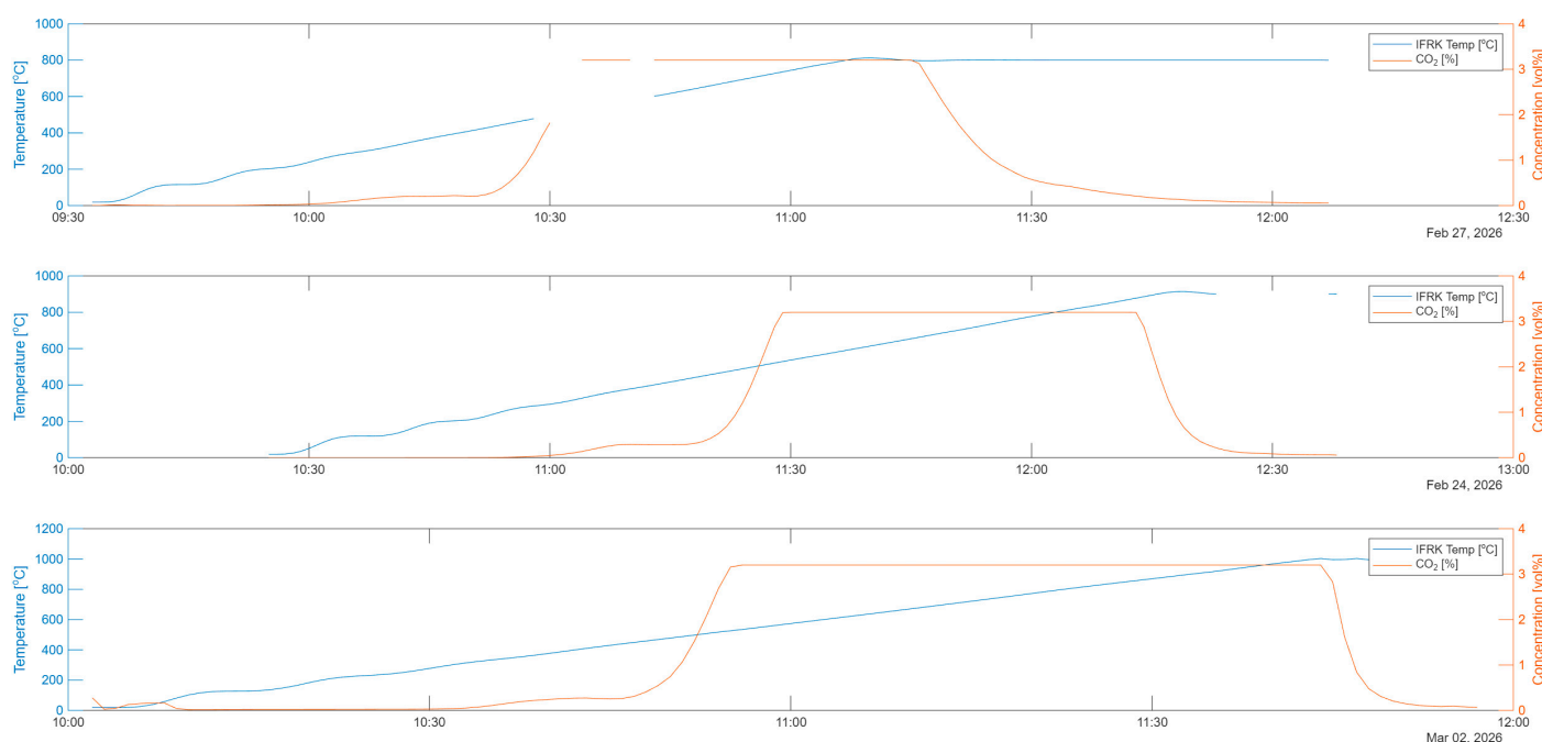
Figure 6. Measured kiln-temperature and outlet- CO_2 concentration profiles during magnesite calcination at setpoint temperatures of 800, 900 and 1000 °C.
