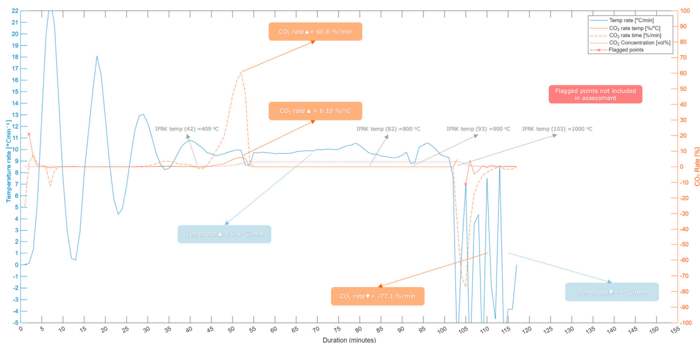
Figure 9. Temperature-rate profile, outlet- \text{CO}_2 concentration and calculated \text{CO}_2 signal slopes for the 1000 ^{\circ}\text{C} magnesite calcination experiment.
