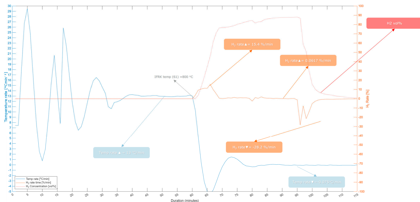
Figure 16. Temperature-rate profile, outlet-H 2 concentration and calculated H 2 signal slopes for Reduction #2, performed with the −2.5 + 1 mm laterite fraction at 800 °C.
