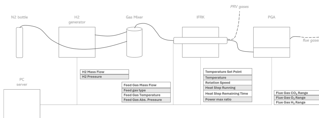
Figure 4. Experimental IFRK platform setup diagram.
