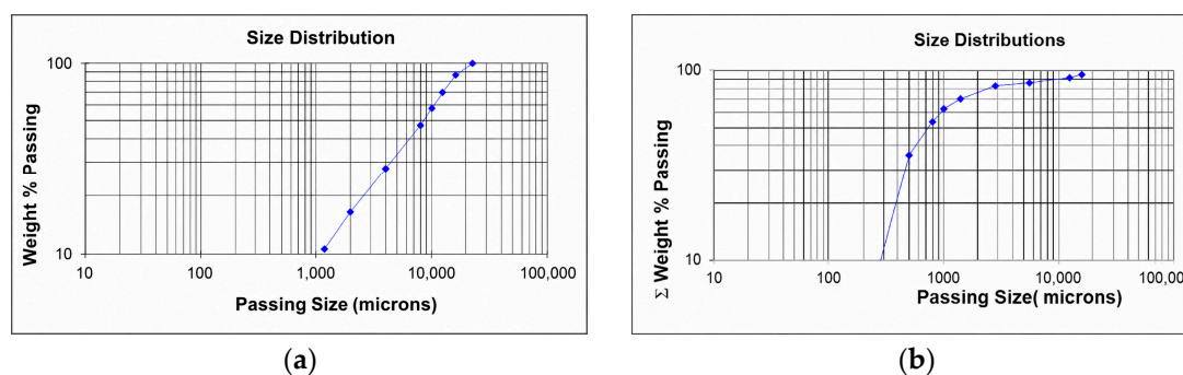
Figure 12. Particle-size distribution of magnesite before and after IFRK calcination: (a) cumulative passing curve of the untreated feed and (b) cumulative passing curve of the calcined product.
