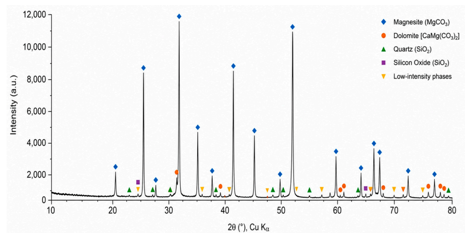
Figure 1. XRD analysis in the feed magnesite sample.
