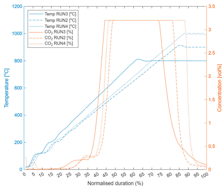
Figure 10. Normalised kiln-temperature and outlet- \text{CO}_2 concentration profiles for the magnesite calcination experiments at 800, 900 and 1000 °C.
