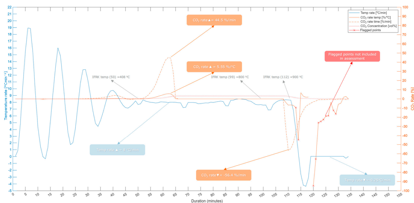
Figure 8. Temperature-rate profile, outlet-CO 2 concentration and calculated CO 2 signal slopes for the 900 °C magnesite calcination experiment.
