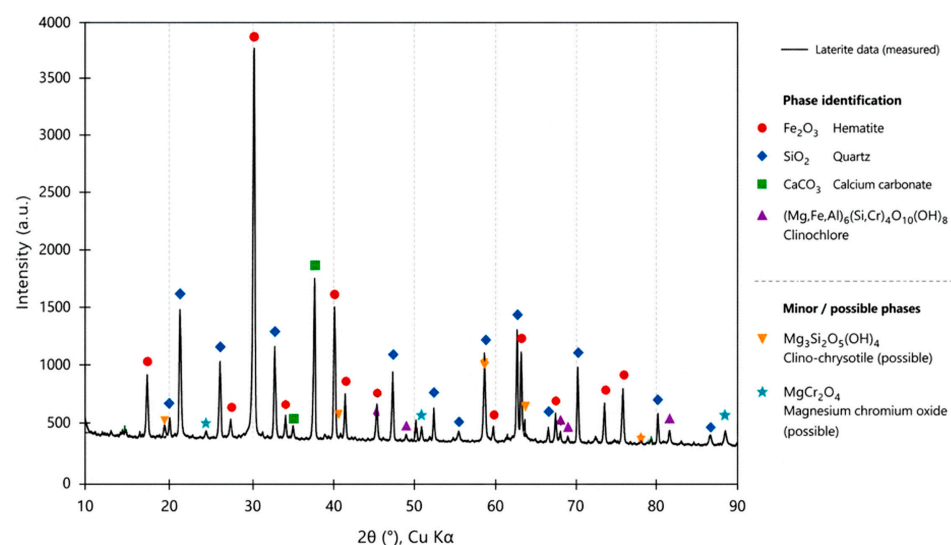
Figure 2. XRD analysis in the lateritic ore sample.
