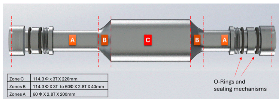
Figure 3. IFRK cylindrical tube simulation in SOLIDWORKS 2026 [31].
