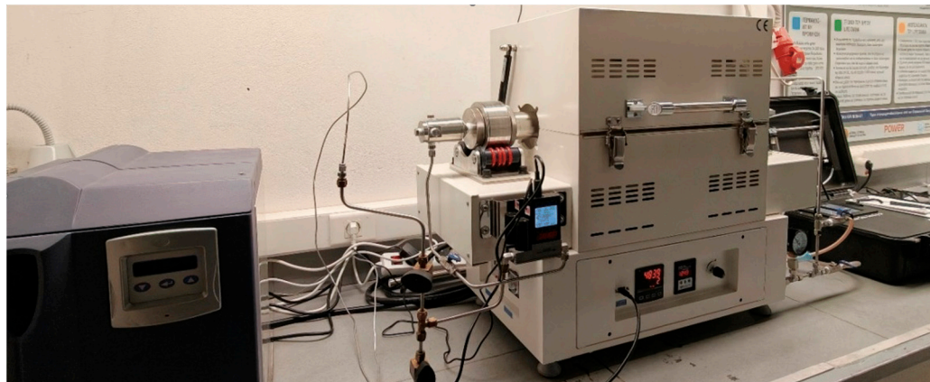
Figure 5. IFRK platform setup.
