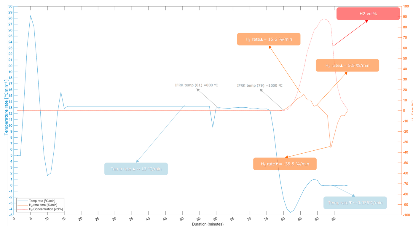
Figure 17. Temperature-rate profile, outlet-H 2 concentration and calculated H 2 signal slopes for Reduction #4, performed with the −2.5 + 1 mm laterite fraction at 1000 °C.
