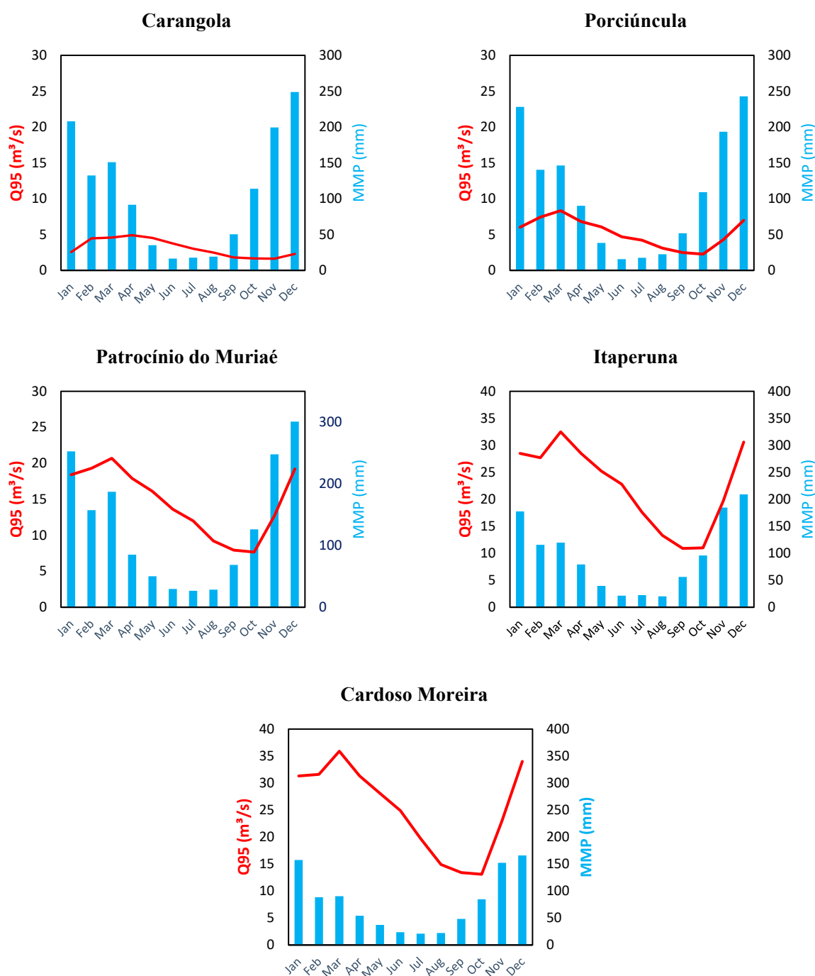
Figure 4. Sazonal variation in Q95 low flow as a function of monthly mean precipitation (MMP) for the monitored stations in the Muriaé River Basin (MRB) during the period 1961–2020.
