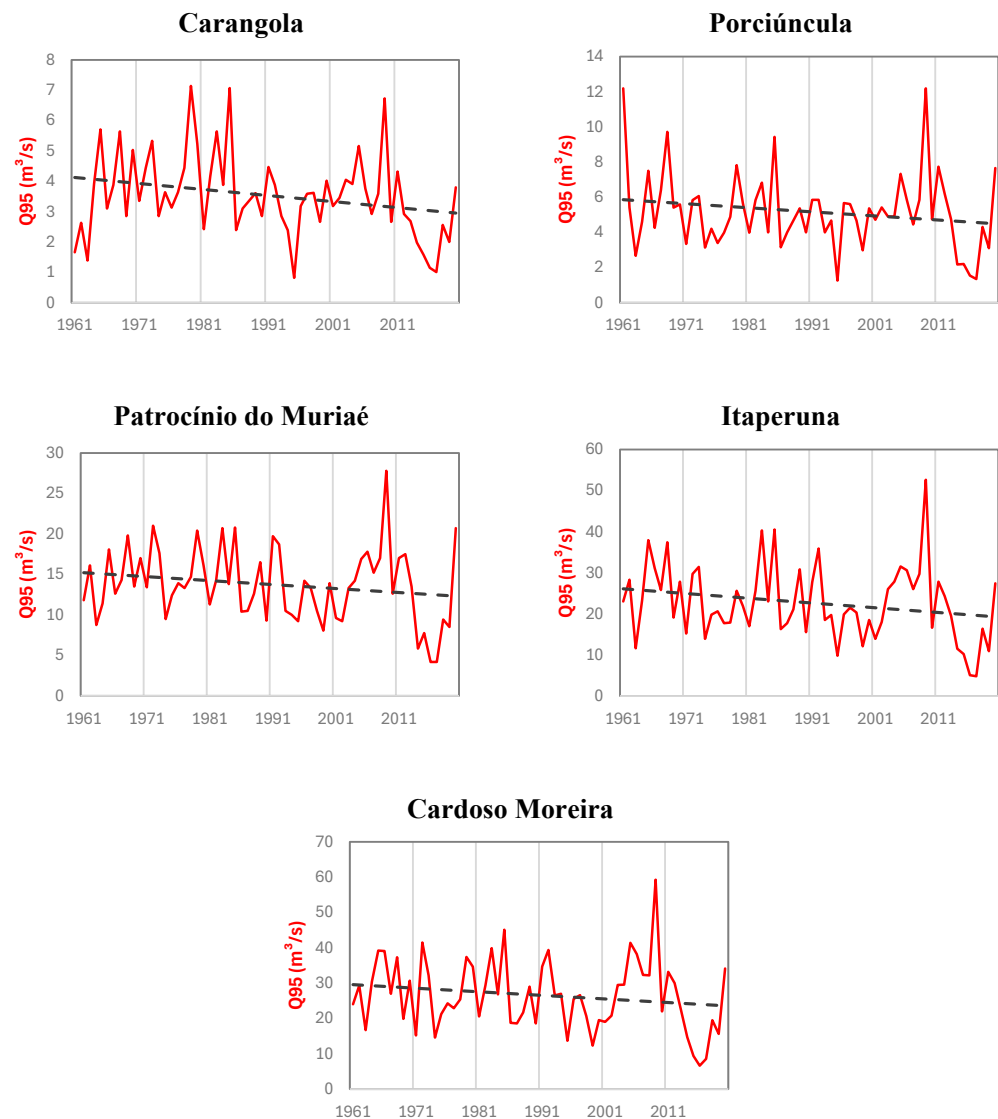
Figure 6. Annual Q95 variability and corresponding linear trend lines for the streamflow monitoring stations in the Muriaé River Basin (MRB) during the period 1961–2020. The figures illustrate the temporal behavior of observed trends in water availability at Carangola, Porciúncula, Patrocínio do Muriaé, Itaperuna, and Cardoso Moreira stations.
