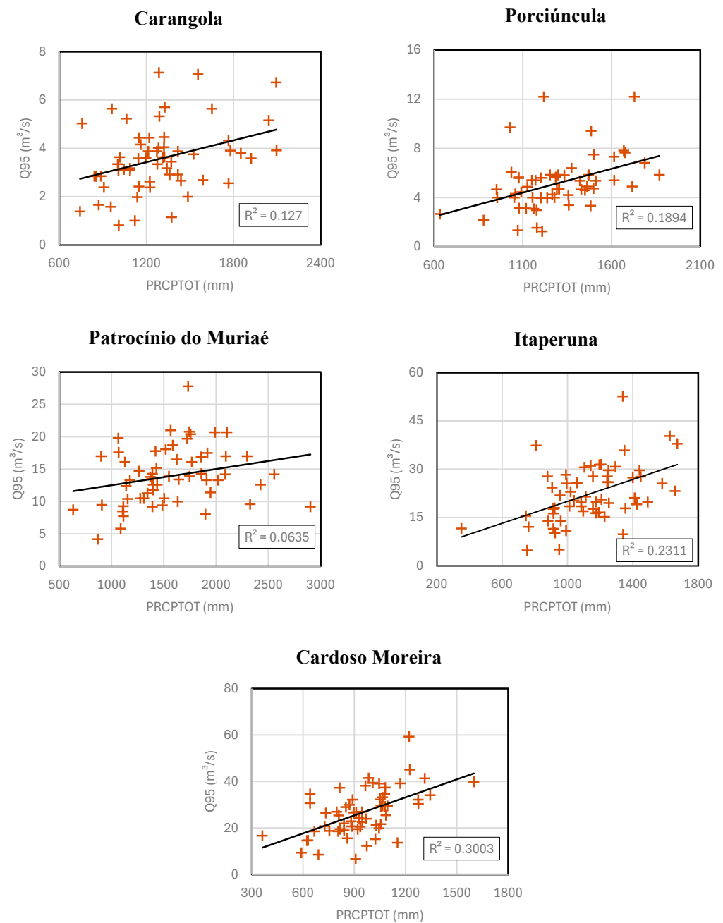
Figure 7. Scatterplots showing the relationship between total annual precipitation (PRCPTOT) and Q95 low flow for the monitored stations in the Muriaé River Basin (MRB) during the period 1961–2020.
