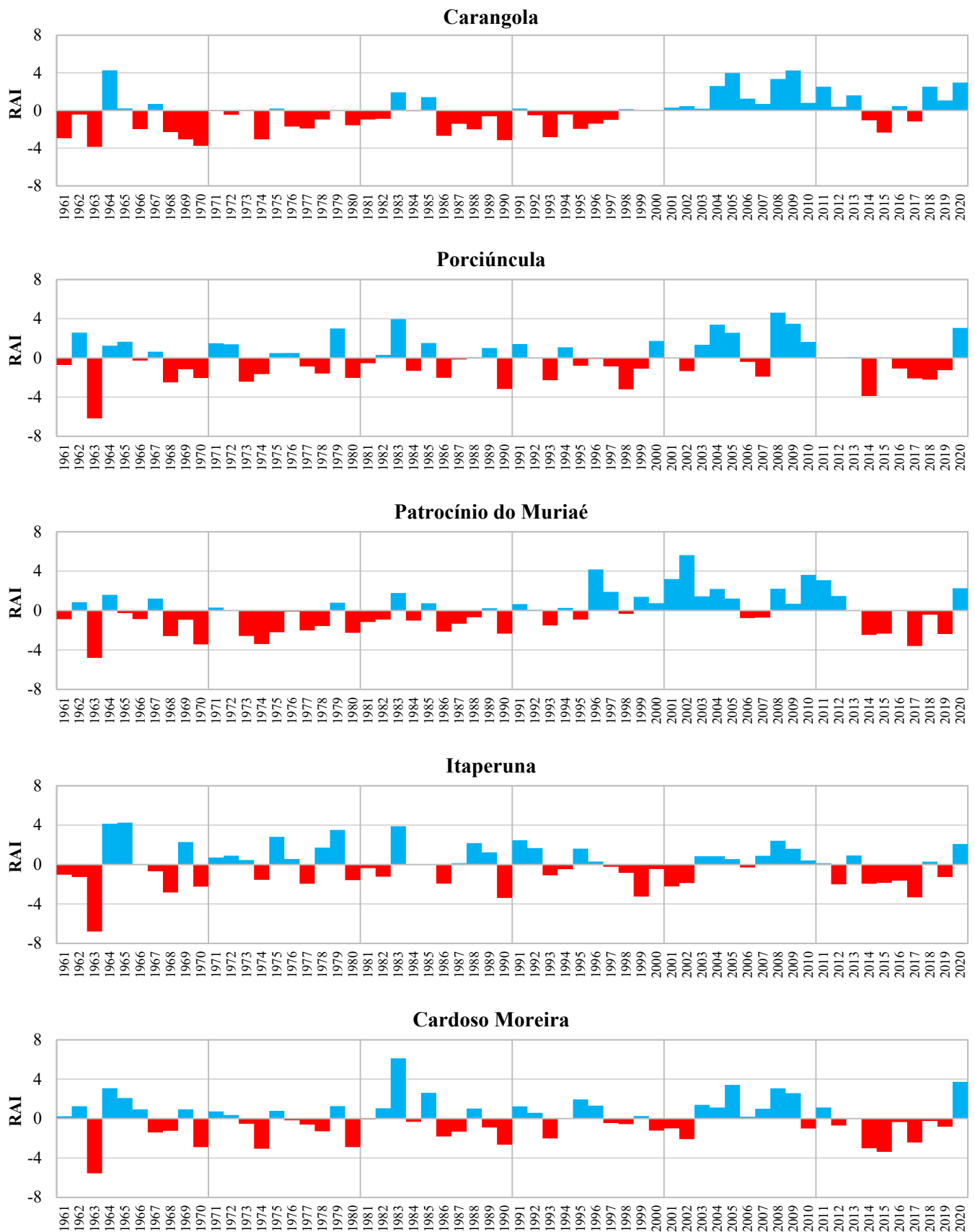
Figure 8. Annual Rainfall Anomaly Index (RAI) for the monitored stations in the Muriaé River Basin (MRB) during the period 1961–2020. Positive values (blue bars) indicate wet conditions, whereas negative values (red bars) indicate dry conditions.
