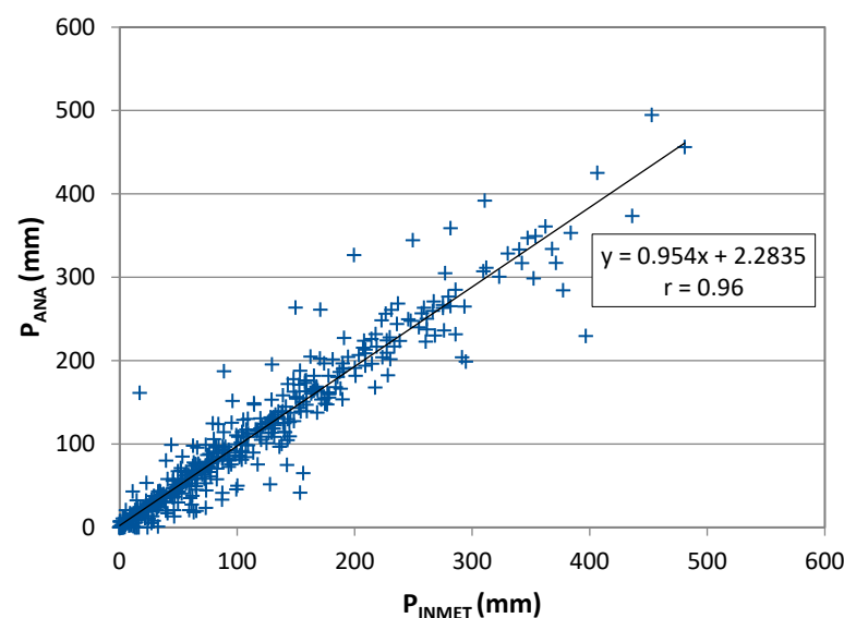
Figure 2. Correlation between monthly mean precipitation (MMP) recorded at the Itaperuna ANA and Itaperuna INMET stations.
