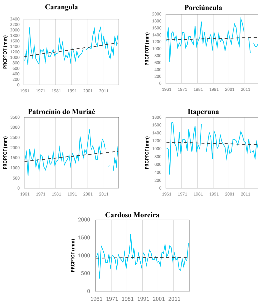
Figure 5. Temporal variability of total annual precipitation (PRCPTOT) and corresponding trend lines for the monitored stations in the Muriaé River Basin (MRB) during the period 1961–2020.
