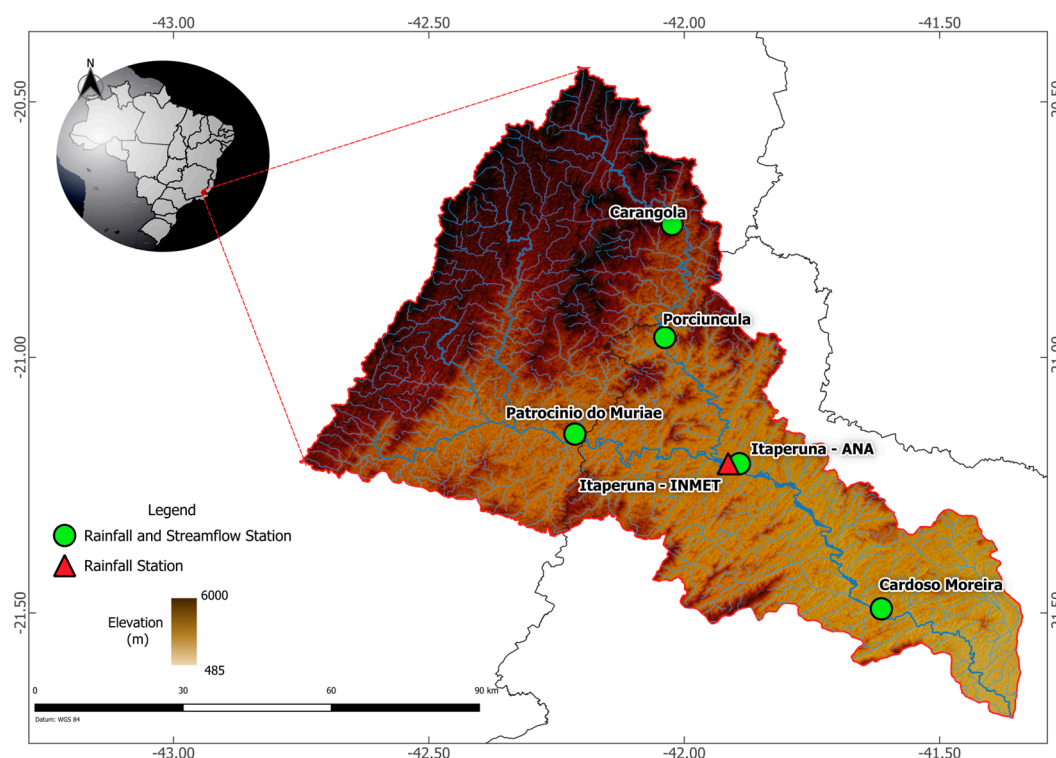
Figure 1. Location of the Muriaé River Basin (MRB) in Southeast Brazil and spatial distribution of the selected rainfall and streamflow monitoring stations used in this study.
