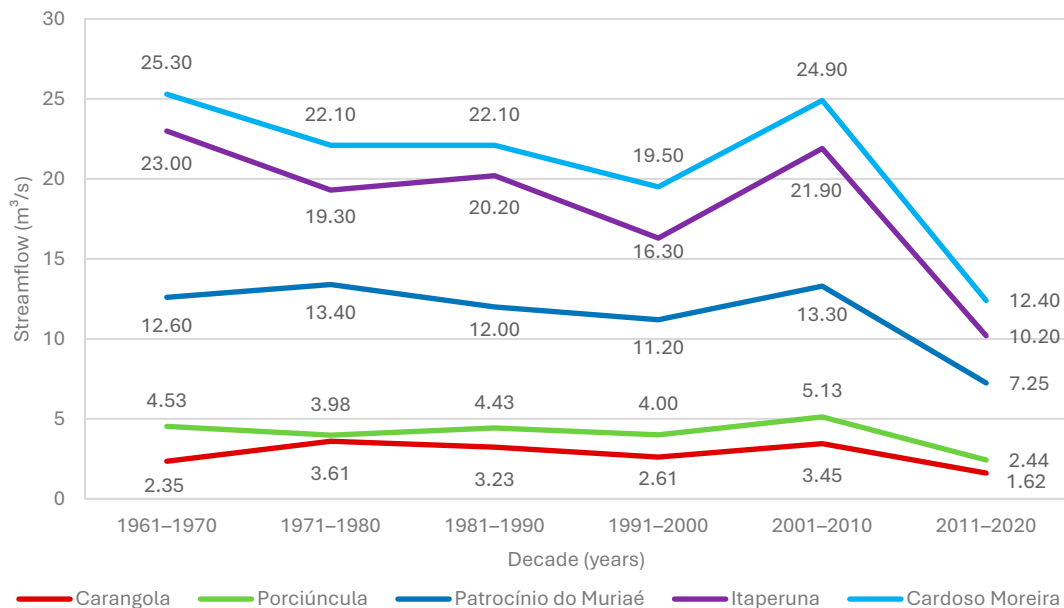
Figure 3. Decadal variation in Q95 low flow for the monitored stations in the Muriaé River Basin (MRB) during the period 1961–2020.
