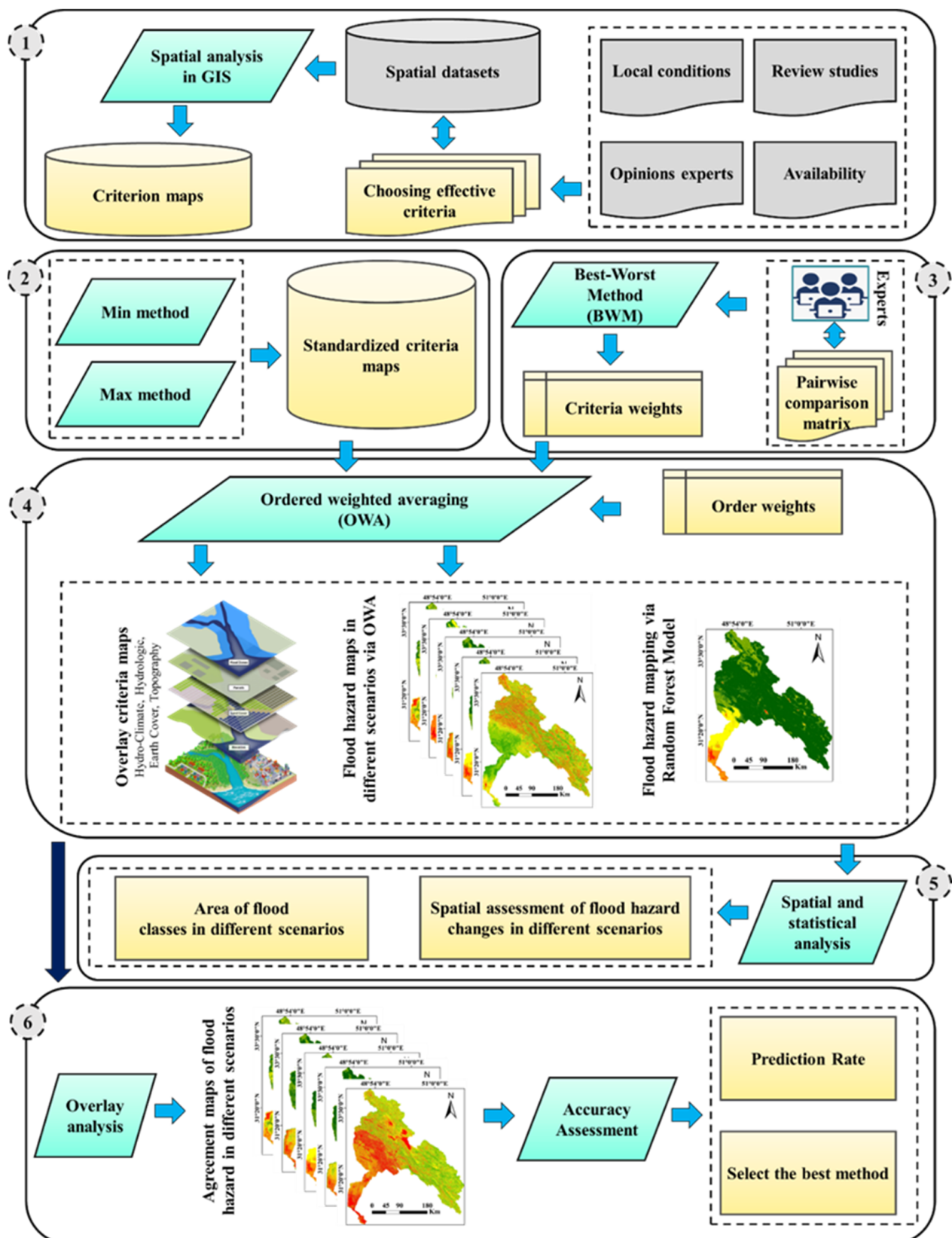
Figure 4. Flowchart of the current research methodology based on the different steps.
