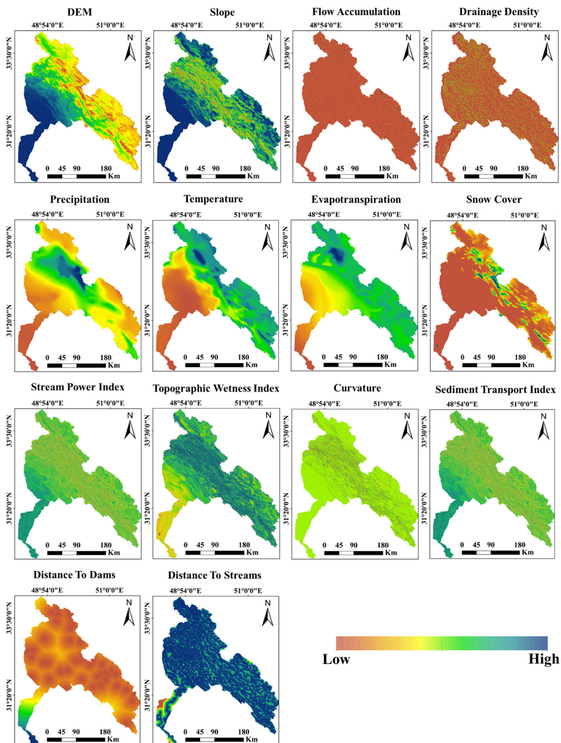
Figure 2. Map of continuous criteria influencing flood susceptibility.
