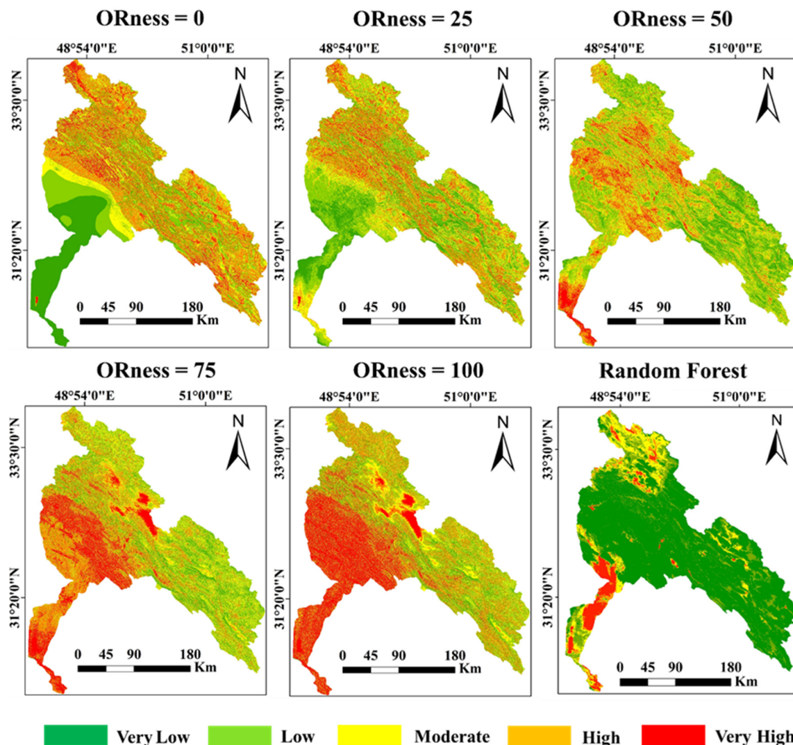
Figure 6. Flood susceptibility prospectively maps for the selected values of ORness and RF model.
