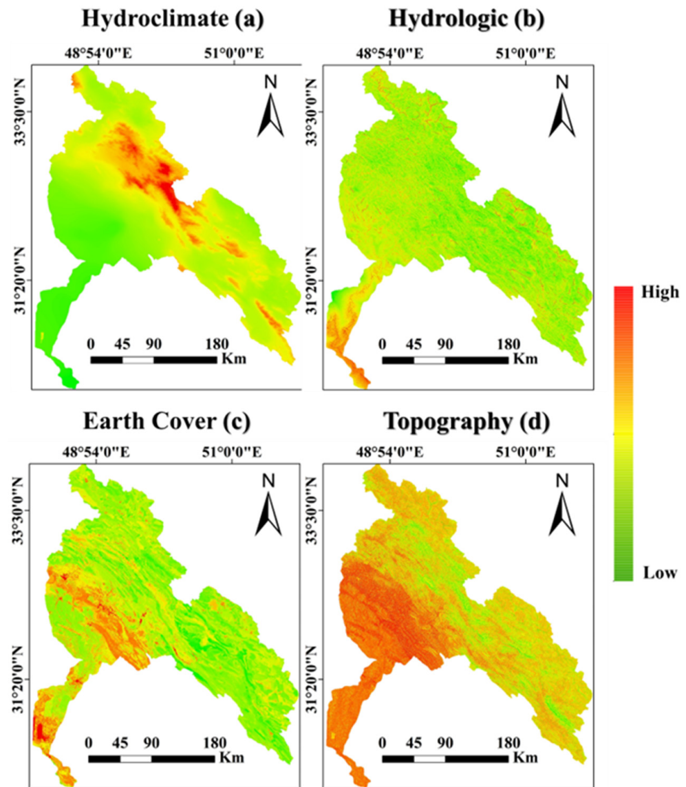
Figure 5. Criteria Integrating Flood susceptibility; Hydro-Climate (a), Hydrologic (b), Earth Cover (c), and Topography (d).
