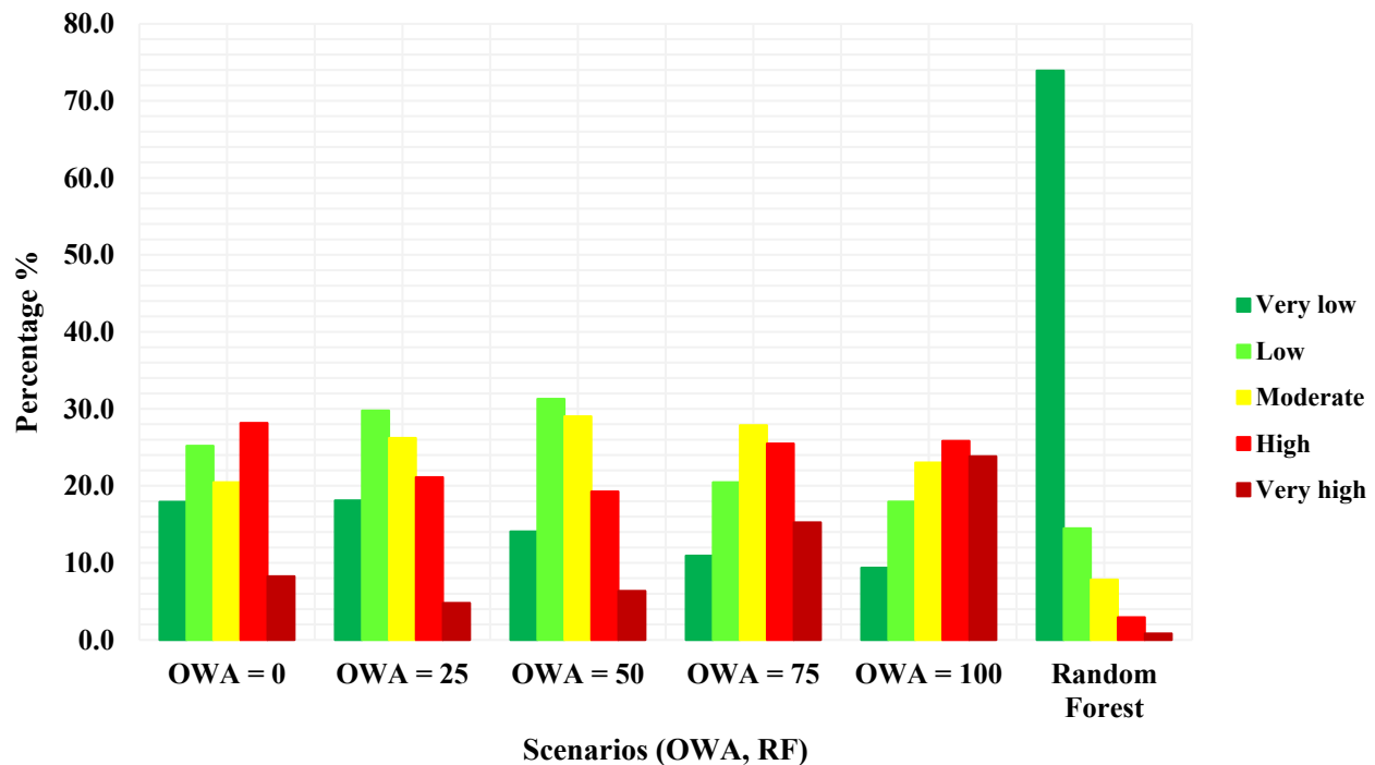
Figure 10. Percentages of actual flood occurrence locations within each flood probability class.
