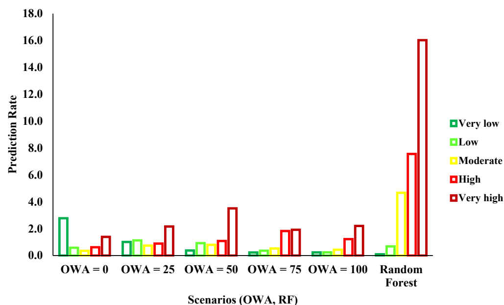
Figure 7. Prediction Rate (PR) for different flood probability classes.
