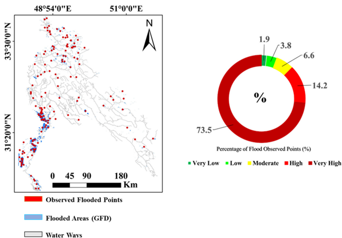
Figure 11. Assessment of field flood points distribution and their correspondence with flood susceptibility classes predicted RF.
