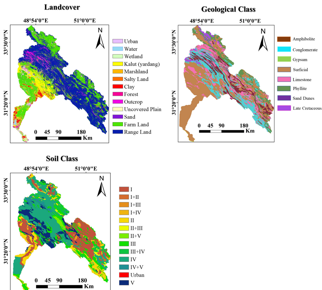
Figure 3. Map of the Earth cover criteria Influencing flood susceptibility.
