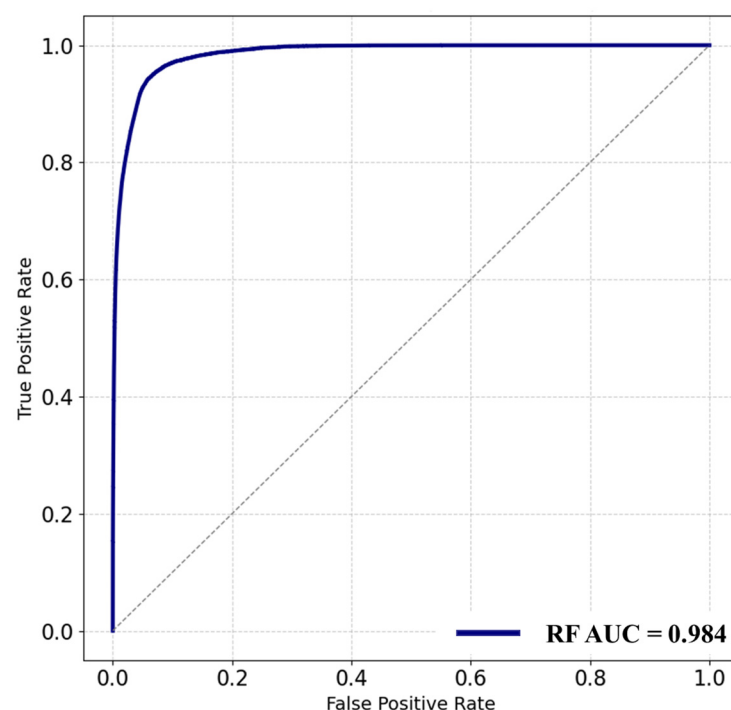
Figure 8. AUC Curve of RF model.
