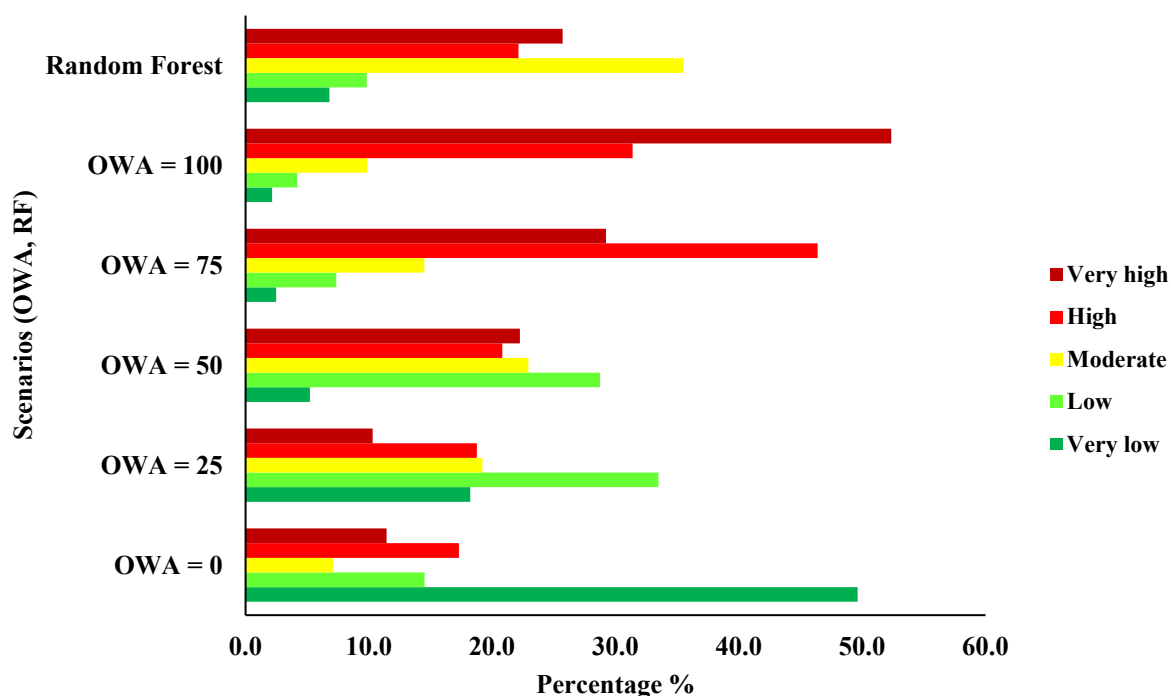
Figure 9. Percentage of the study area assigned to each flood probability class—Class area (%).
