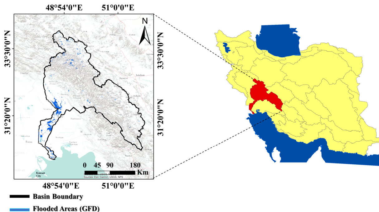
Figure 1. The study area for the current research.
