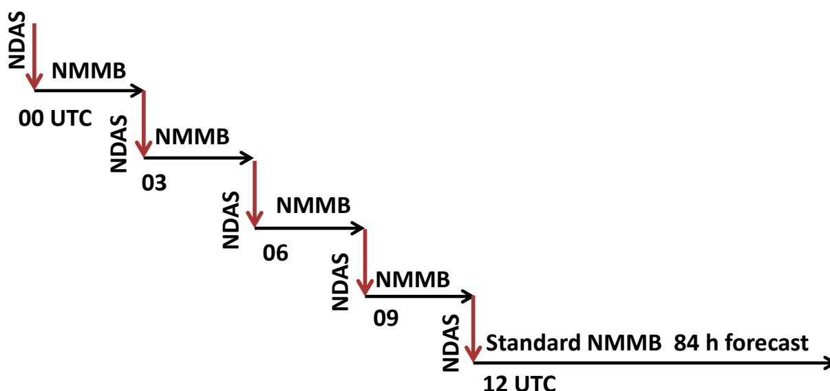
Figure 2. Schematic diagram of four sequences of the NDAS and NMMB short forecasts to prepare initialization condition for a standard 12 UTC cycle NAM forecast.
