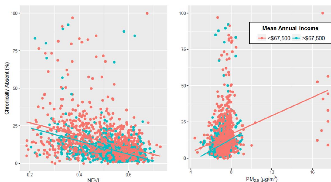
Figure 2. Relationship between NDVI and PM 2.5 on the percent of students chronically absent during the 2012–2013 academic year at each school in Massachusetts (USA), stratified by counties with a mean annual income above and below $67,500.
