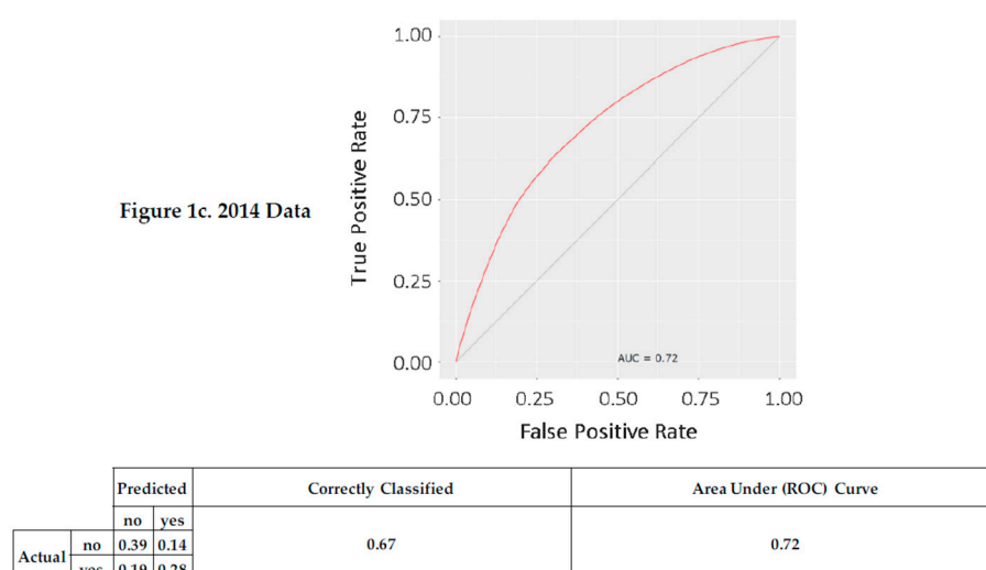
Figure 1. Confusion matrix and area under the receiver operating characteristic curve.
