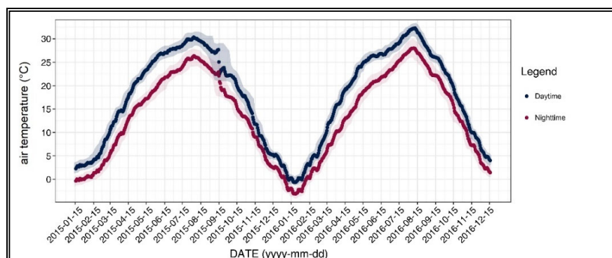
Figure 2. Air temperature of the 31-day moving average.
