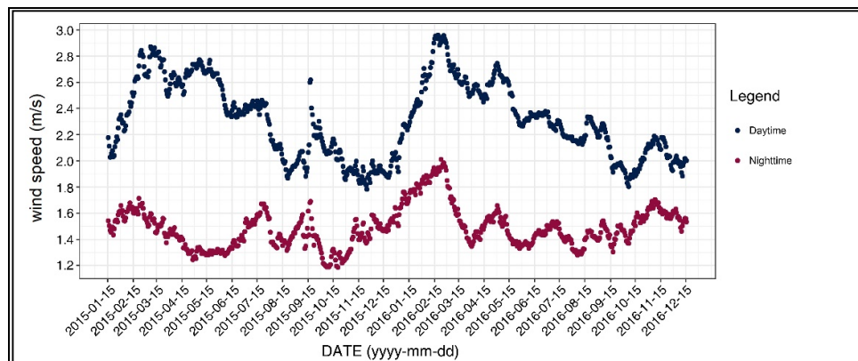
Figure 3. Wind speed of the 31-day moving average.
