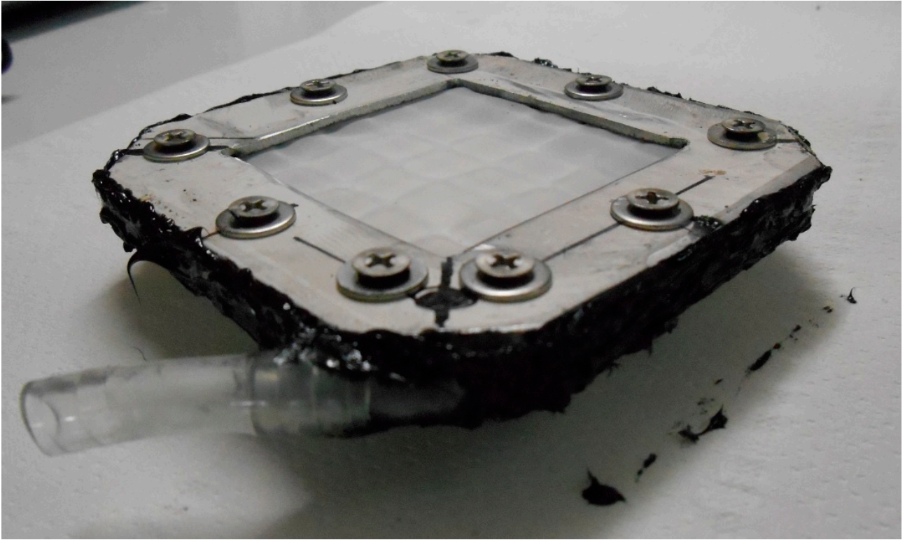
Figure S1. Flat sheet configuration of the nylon support in the SFD MBR module.
