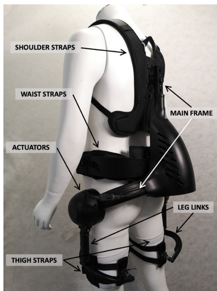
Figure 1. XoTrunk prototype.
