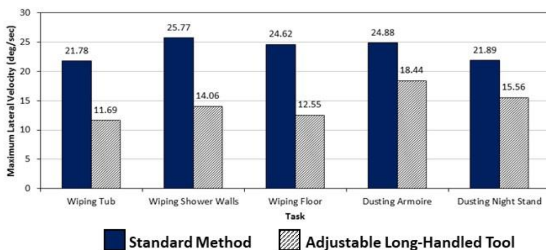
Figure 5. Differences in average maximum lateral trunk velocities between cleaning methods of five bathroom and furniture cleaning methods. All were significantly different ( p < 0.05 ).
