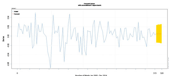
Figure S1. EGARCH models of market volatility and forecasts.
