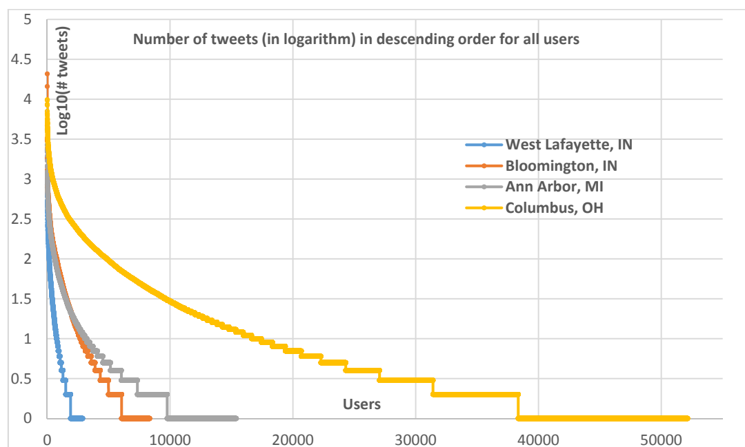
Figure 5. Number of tweets (in logarithm) in descending order for all users.
