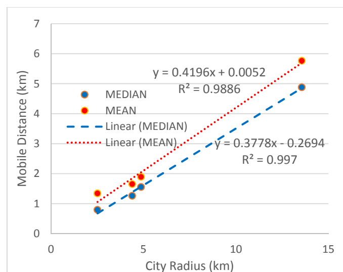
Figure 7. Relationship between city radius and users' average mobile distance.
