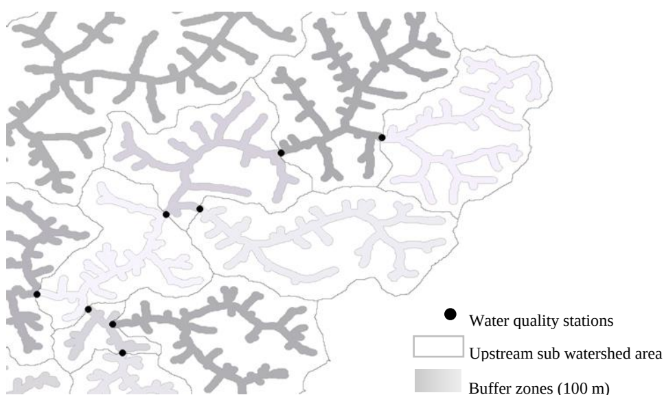
Figure 3. Upstream area delineation and their respective buffer zones in tones of gray. The solid circles are water quality stations (sites).
