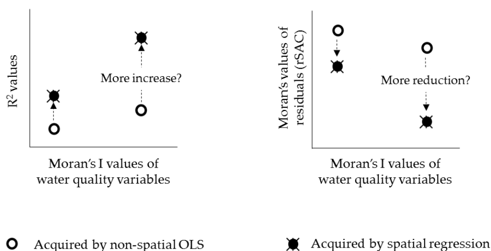
Figure 4. Evaluation of the hypothesis—Moran's I values of the water quality variables appear on the x -axis, and the model outcomes, R^2 and residual SAC, appear on the y -axis. After spatial regression, water quality variables with a higher amount of spatial autocorrelation (SAC) were hypothesized to exhibit improved hydrologic modeling (i.e., more increases in R^2 and more decreases in residual SAC) than those with lower SAC.
