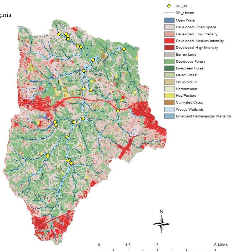
Figure A1. Water stations organization in the stream network and land cover characteristics of each study area. Idaho (a); Kansas (b); Iowa (c); Delaware (d); California (e); Virginia (f); Arizona (g); Colorado (h); Louisiana (i); and Kentucky (j).
