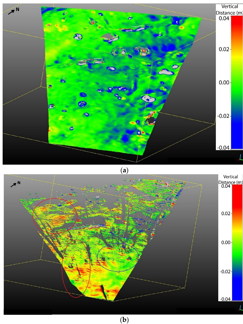
Figure 8. S2 M3C2-difference (m) point cloud of UAV (a) and TLS-derived (b) data in 4 month analysis (19.10.2019–23.02.2020).
