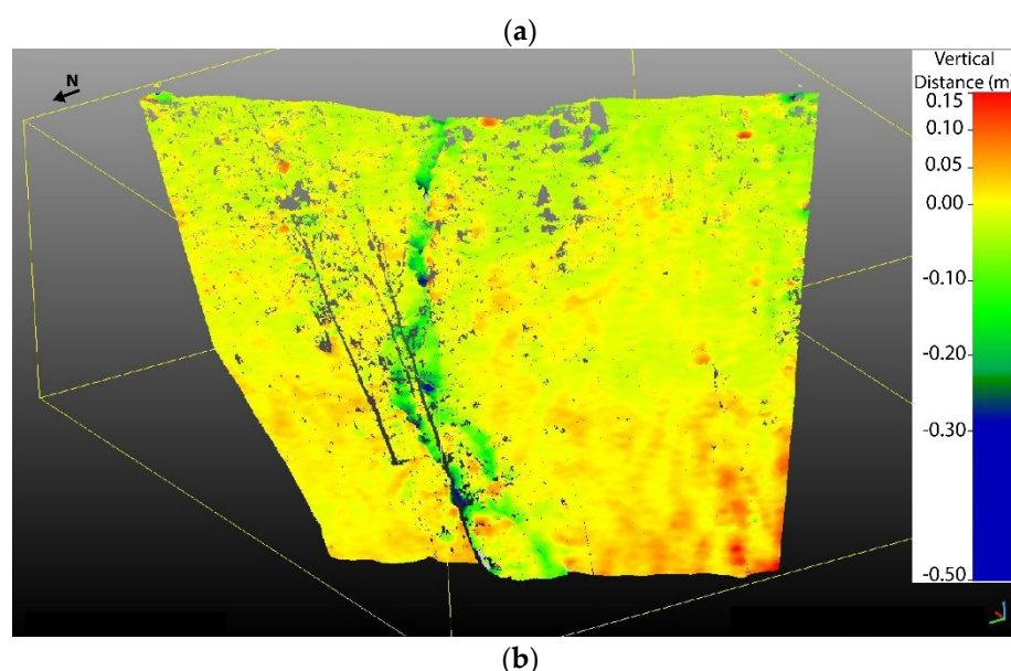
Figure 9. S1 M3C2-difference (m) point cloud of UAV (a) and TLS-derived (b) data in 8 month analysis (23.02.2020–11.10.2020).
