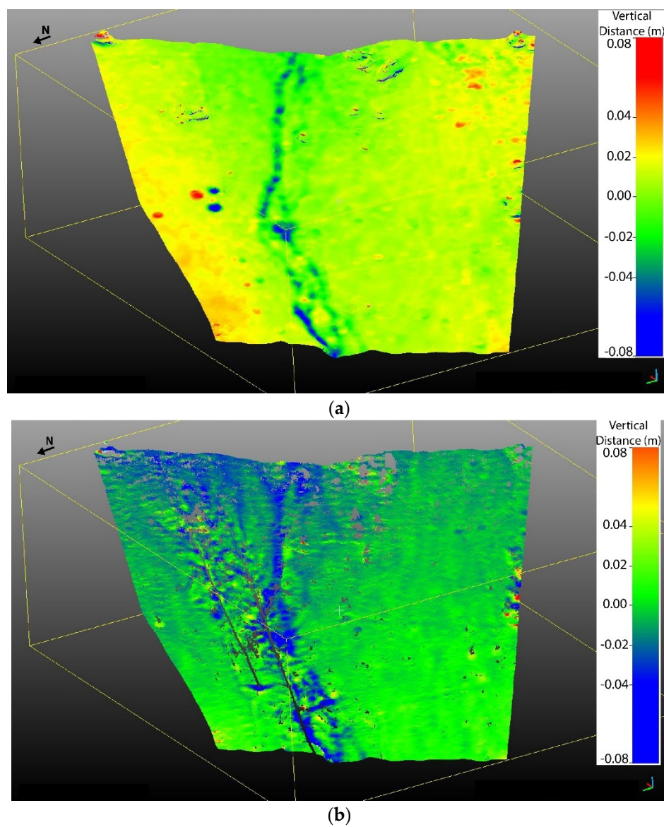
Figure 7. S1 M3C2-difference (m) point cloud of UAV (a) and TLS-derived (b) data in 4 month analysis (19.10.2019–23.02.2020).
