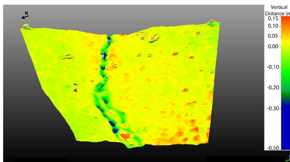
Figure 8. S2 M3C2-difference (m) point cloud of UAV (a) and TLS-derived (b) data in 4 month analysis (19.10.2019–23.02.2020).
