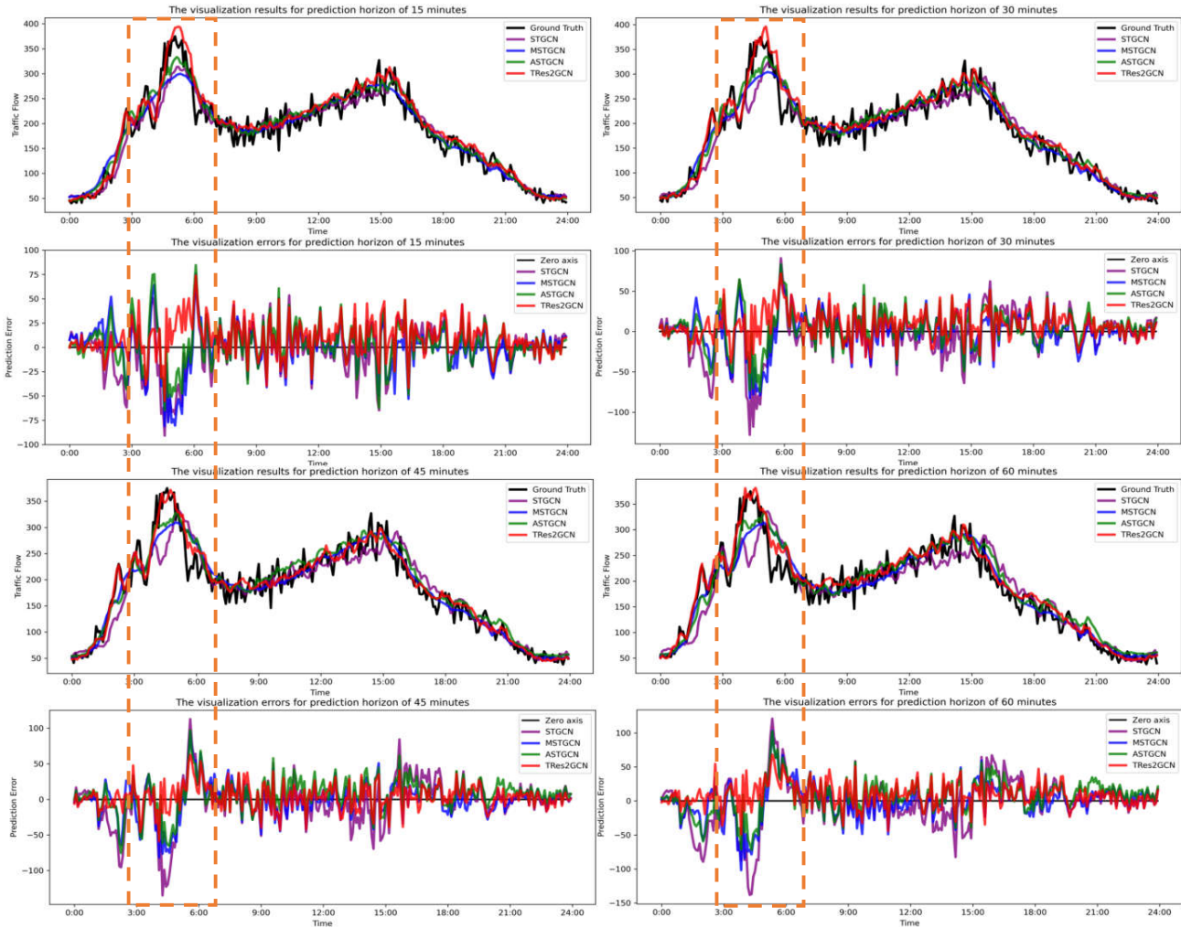
Figure 5. Visualization of prediction results and errors ranging 0–60-min span of sensor #149
