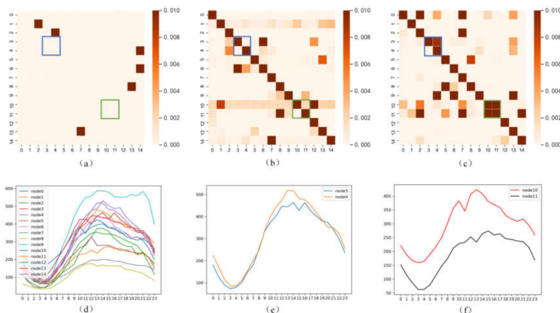
Figure 6. Part of the adjacency matrix at different scales and hourly average traffic flow variation (with PeMS08 as an example). (a) Predefined adjacency matrix. (b) Self-adaptive adjacency matrix at a single scale. (c) Self-adaptive adjacency matrix at multiple scales. (d) Hourly flow variation for the first fifteen nodes. (e) Hourly traffic variation of node 3 and node 4. (f) Hourly traffic variation of node 10 and node 11.
