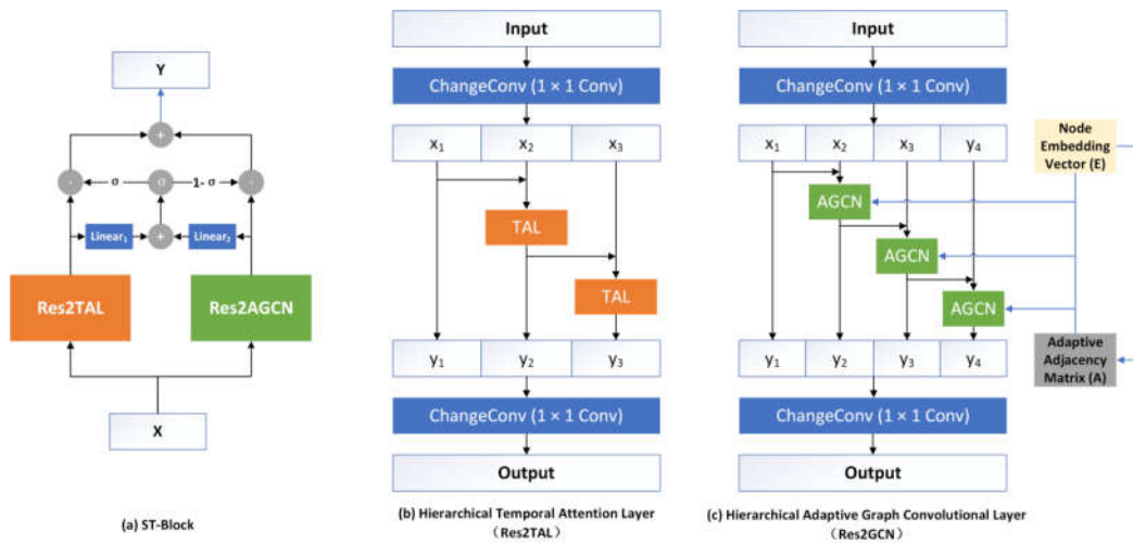
Figure 2. The (a) ST Block of TRes2GCN. The framework of (b) hierarchical temporal attention layer and (c) hierarchical adaptive graph convolution layer.
