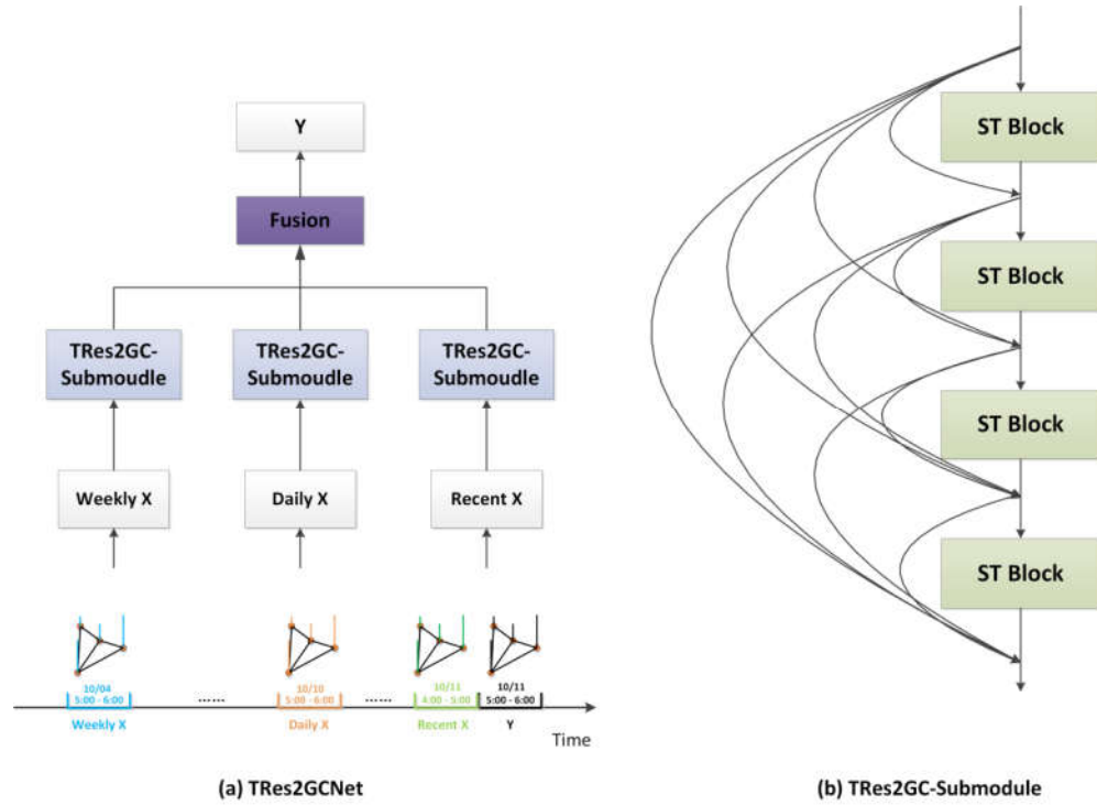
Figure 1. The framework of (a) TRes2GCNet and (b) TRes2GC-Submodule.
