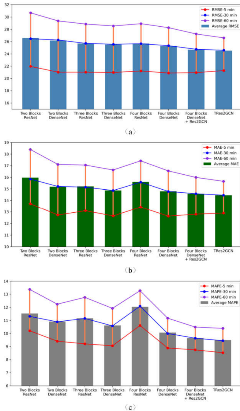
Figure 4. Visualization of the impact of components on the prediction error (PeMS08 as an example), (a) RMSE, (b) MAE and (c) MAPE; the error bars represent the floating changes of the predicted metrics in 60 min; the red line represents the outcome metrics predicted in 5 min; the blue line represents the outcome metrics predicted in 30 min; the purple line represents the outcome metrics predicted in 60 min.
