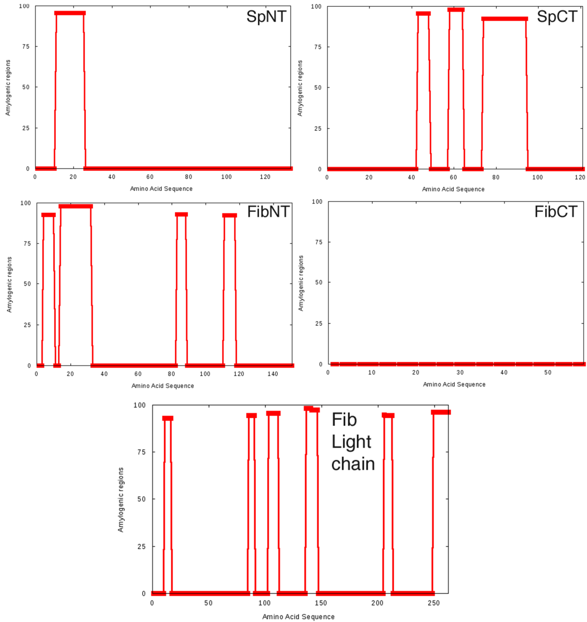
Figure S1. Waltz plots of spidroin NT (SpNT), spidroin CT (SpCT), fibroin heavy chain NT (FibNT), fibroin heavy chain CT (FibCT) and fibroin light chain.
