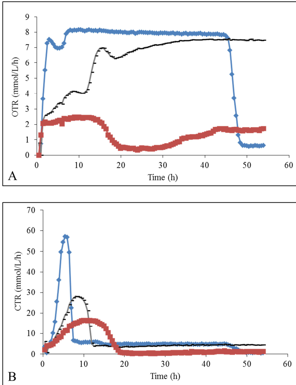
Fig. S1. Oxygen Transfer Rate OTR (A) and Carbon dioxide Transfer Rate CTR (B) of K. marxianus grown in: ◆ YMD; ■ YMD + 0.5% [Emim][OAc]; ■ YMD + 1% [Emim][OAc]. The results are mean of two repetitions. Error bars are not represented to avoid overloading the figure.
